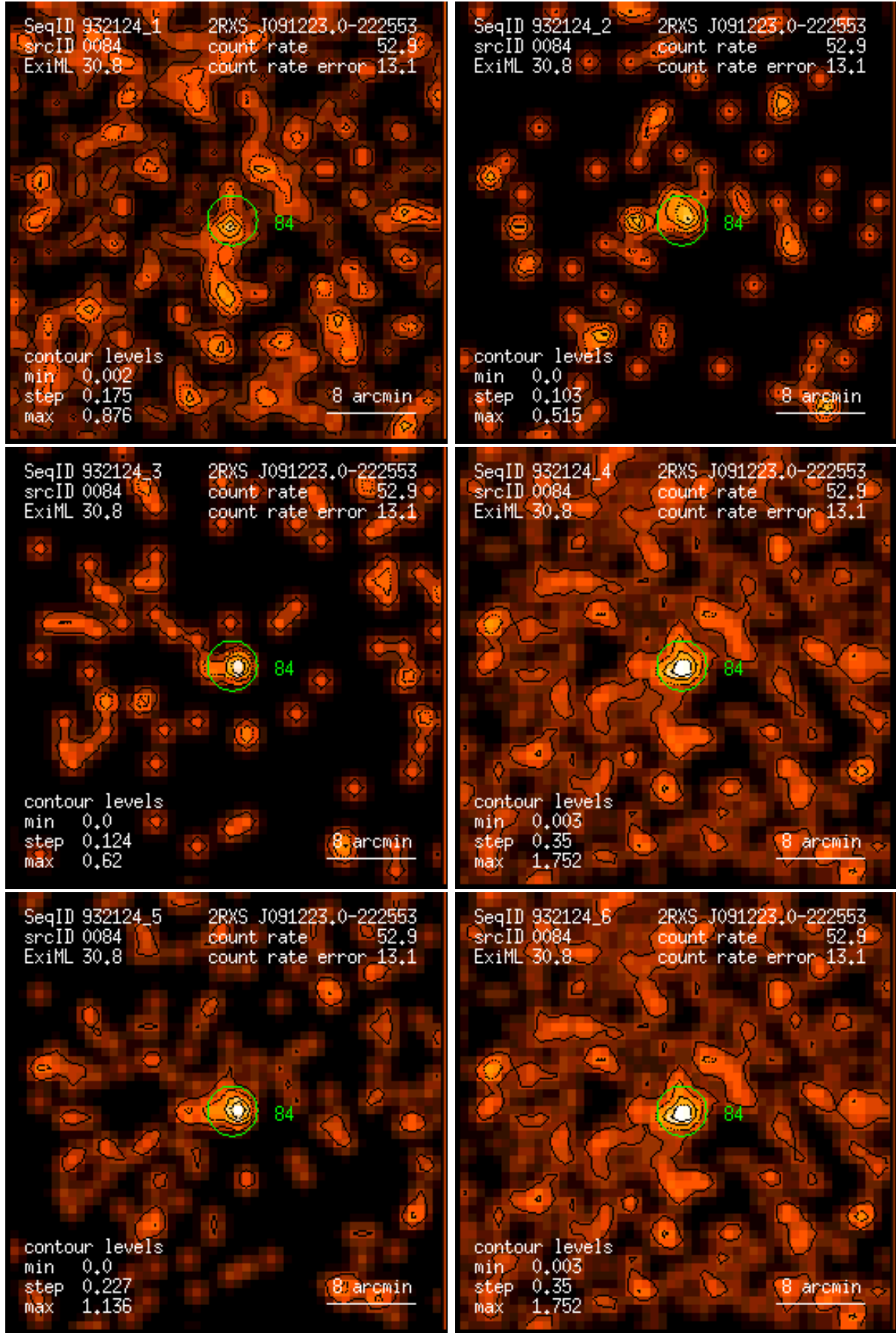
Figure 84: RASS 932124: detection 0084: band rate images, Gaussian filter: (1) PSPC channels 11 – 41, (2) 52 – 90, (3) 91 – 201, (4) 11 – 235, (5) 52 – 201, (6) 11 – 201. Broad band rates in counts/ks. Band rate contour levels in counts/ks/arcmin 2 .
