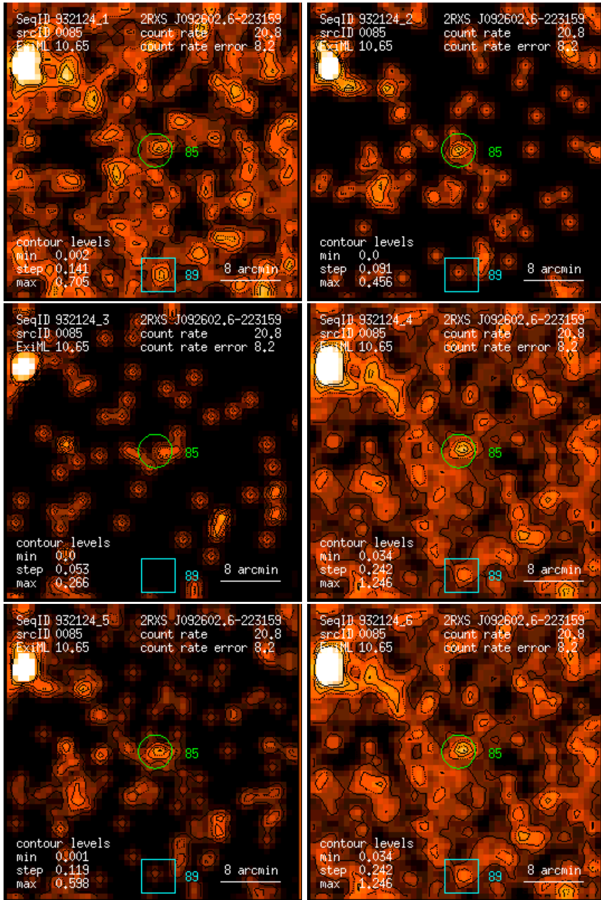
Figure 85: RASS 932124: detection 0085: band rate images, Gaussian filter: (1) PSPC channels 11 – 41, (2) 52 – 90, (3) 91 – 201, (4) 11 – 235, (5) 52 – 201, (6) 11 – 201. Broad band rates in counts/ks. Band rate contour levels in counts/ks/arcmin 2 .
