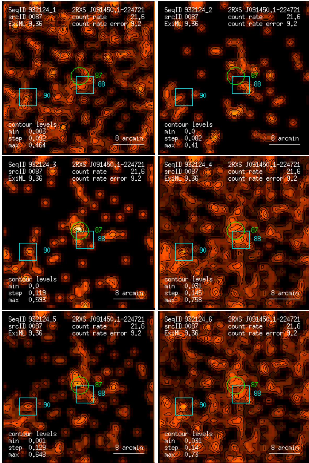
Figure 87: RASS 932124: detection 0087: band rate images, Gaussian filter: (1) PSPC channels 11 – 41, (2) 52 – 90, (3) 91 – 201, (4) 11 – 235, (5) 52 – 201, (6) 11 – 201. Broad band rates in counts/ks. Band rate contour levels in counts/ks/arcmin 2 .
