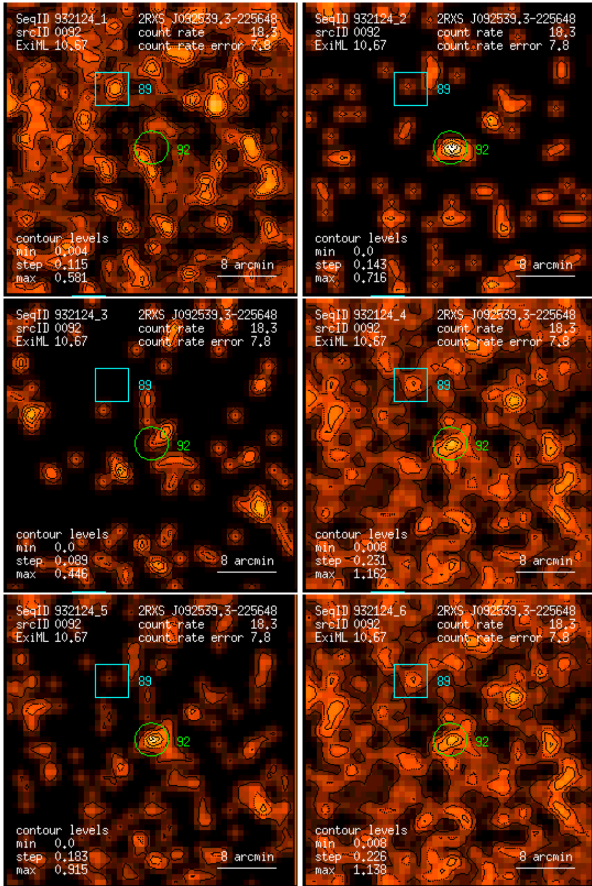
Figure 92: RASS 932124: detection 0092: band rate images, Gaussian filter: (1) PSPC channels 11 – 41, (2) 52 – 90, (3) 91 – 201, (4) 11 – 235, (5) 52 – 201, (6) 11 – 201. Broad band rates in counts/ks. Band rate contour levels in counts/ks/arcmin 2 .
