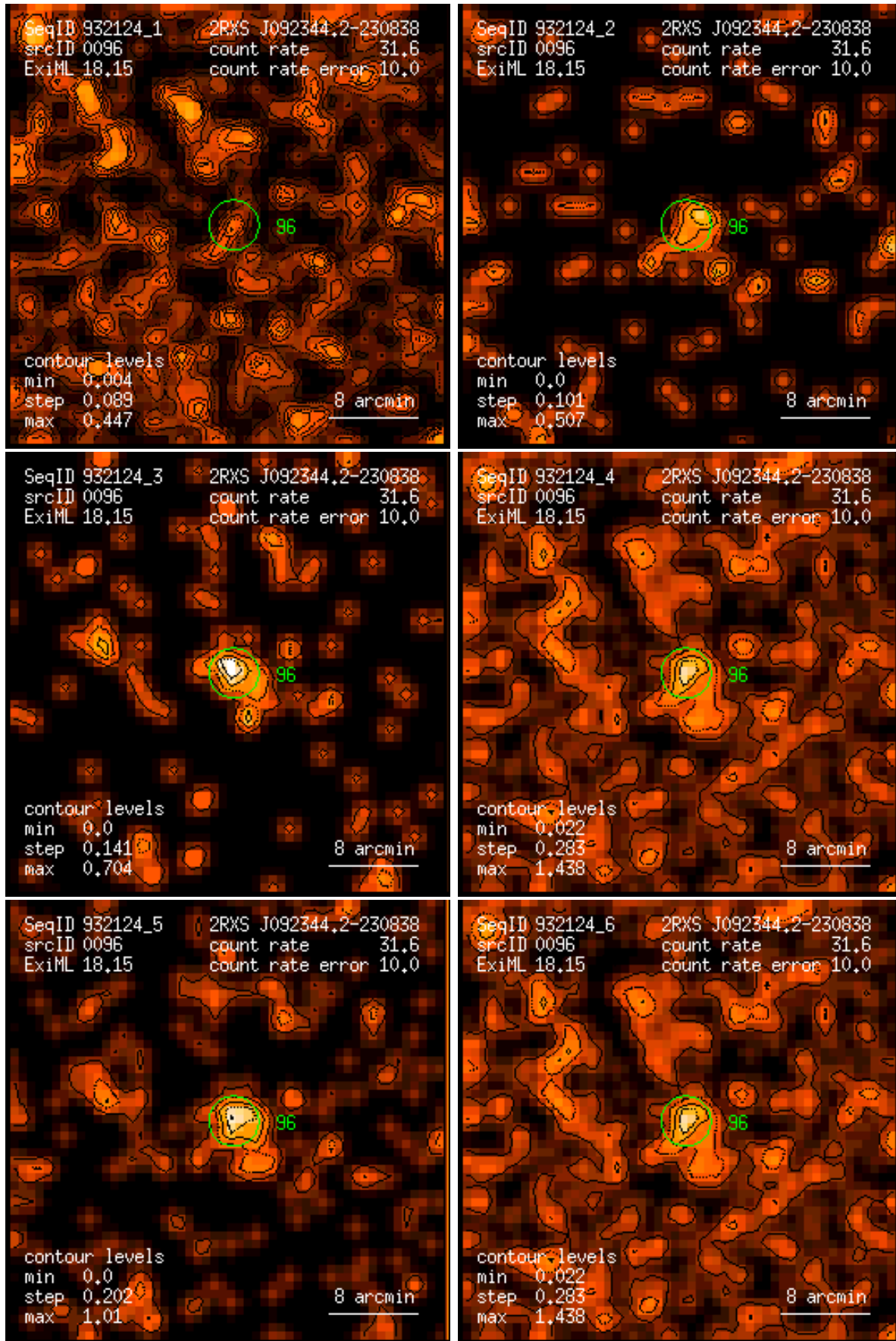
Figure 96: RASS 932124: detection 0096: band rate images, Gaussian filter: (1) PSPC channels 11 – 41, (2) 52 – 90, (3) 91 – 201, (4) 11 – 235, (5) 52 – 201, (6) 11 – 201. Broad band rates in counts/ks. Band rate contour levels in counts/ks/arcmin 2 .
