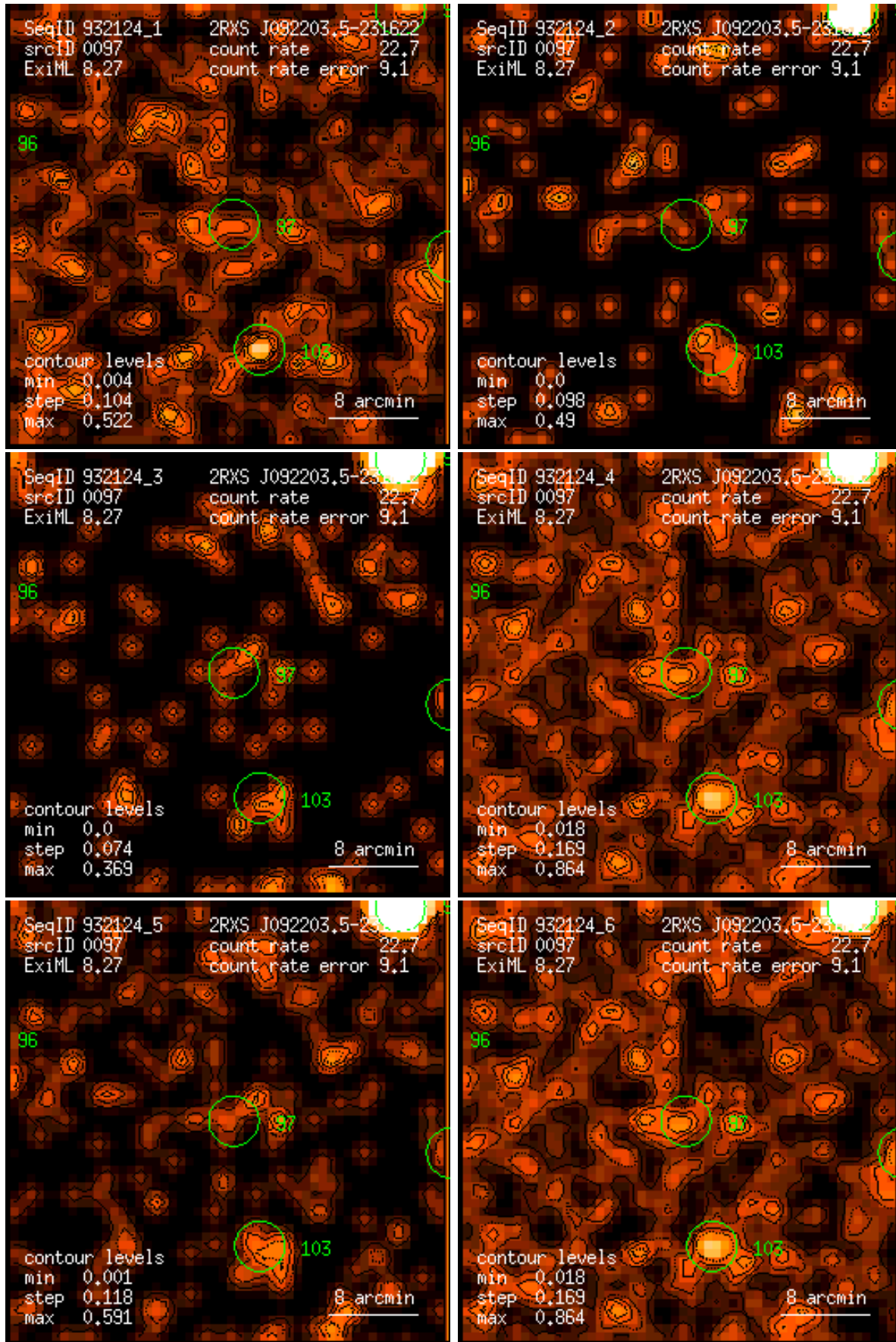
Figure 97: RASS 932124: detection 0097: band rate images, Gaussian filter: (1) PSPC channels 11 – 41, (2) 52 – 90, (3) 91 – 201, (4) 11 – 235, (5) 52 – 201, (6) 11 – 201. Broad band rates in counts/ks. Band rate contour levels in counts/ks/arcmin 2 .
