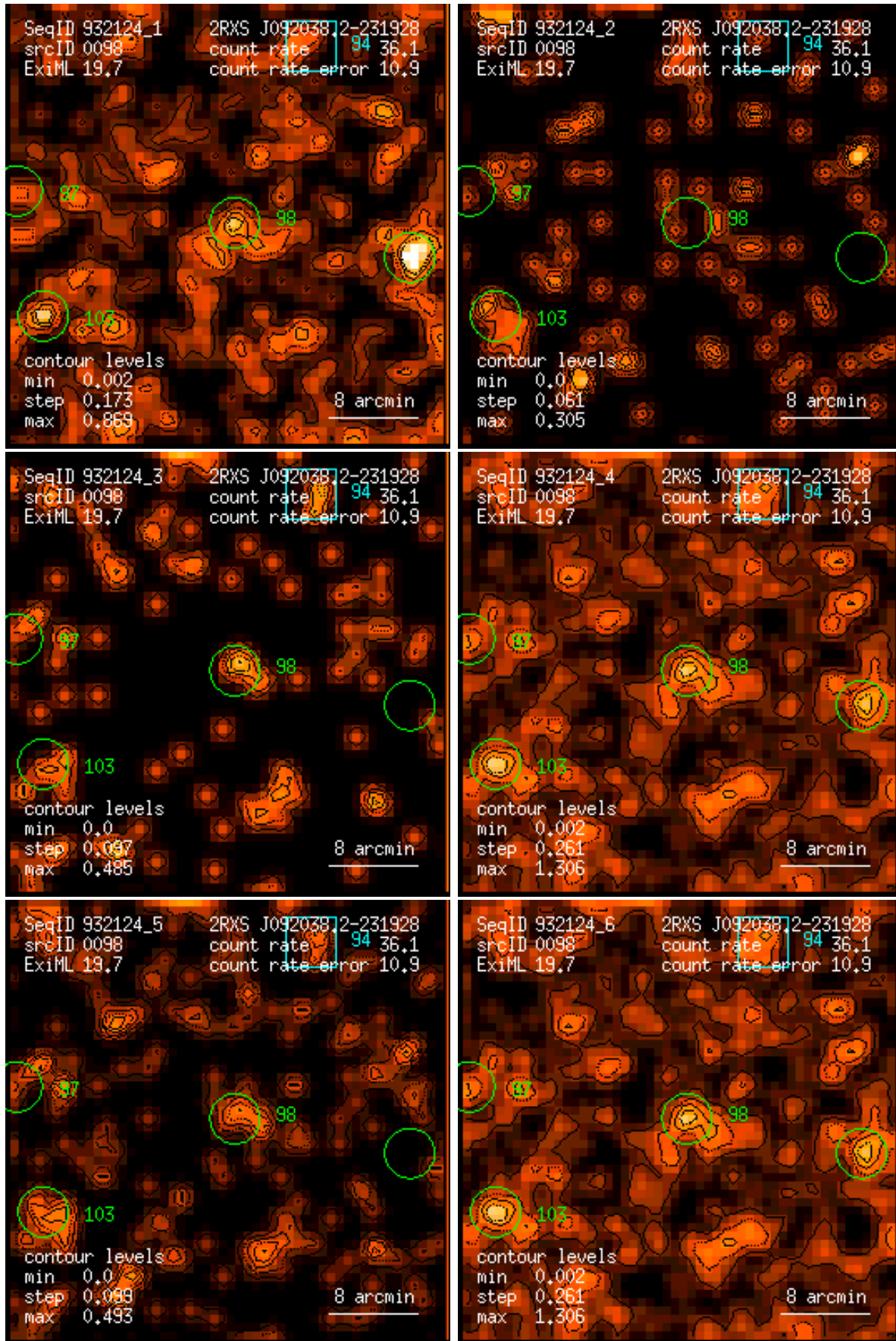
Figure 98: RASS 932124: detection 0098: band rate images, Gaussian filter: (1) PSPC channels 11 – 41, (2) 52 – 90, (3) 91 – 201, (4) 11 – 235, (5) 52 – 201, (6) 11 – 201. Broad band rates in counts/ks. Band rate contour levels in counts/ks/arcmin 2 .
