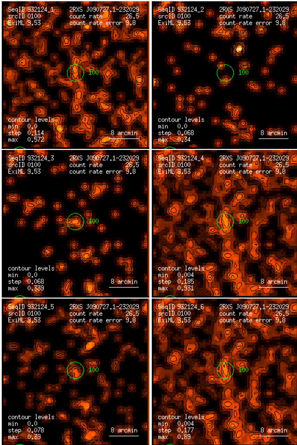
Figure 100: RASS 932124: detection 0100: band rate images, Gaussian filter: (1) PSPC channels 11 – 41, (2) 52 – 90, (3) 91 – 201, (4) 11 – 235, (5) 52 – 201, (6) 11 – 201. Broad band rates in counts/ks. Band rate contour levels in counts/ks/arcmin 2 .
