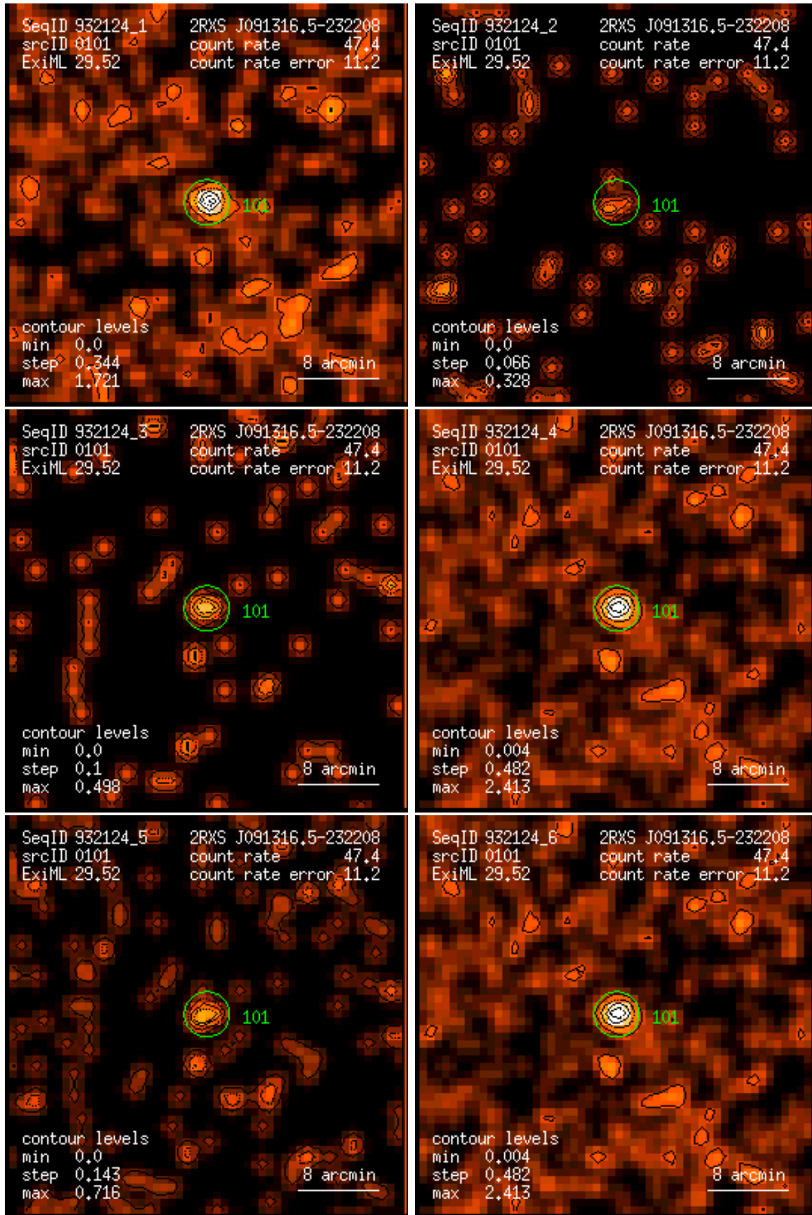
Figure 101: RASS 932124: detection 0101: band rate images, Gaussian filter: (1) PSPC channels 11 – 41, (2) 52 – 90, (3) 91 – 201, (4) 11 – 235, (5) 52 – 201, (6) 11 – 201. Broad band rates in counts/ks. Band rate contour levels in counts/ks/arcmin 2 .
