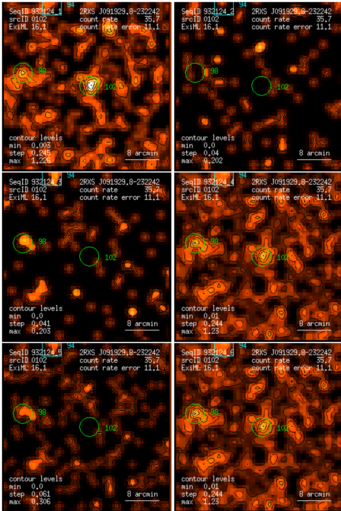
Figure 102: RASS 932124: detection 0102: band rate images, Gaussian filter: (1) PSPC channels 11 – 41, (2) 52 – 90, (3) 91 – 201, (4) 11 – 235, (5) 52 – 201, (6) 11 – 201. Broad band rates in counts/ks. Band rate contour levels in counts/ks/arcmin 2 .
