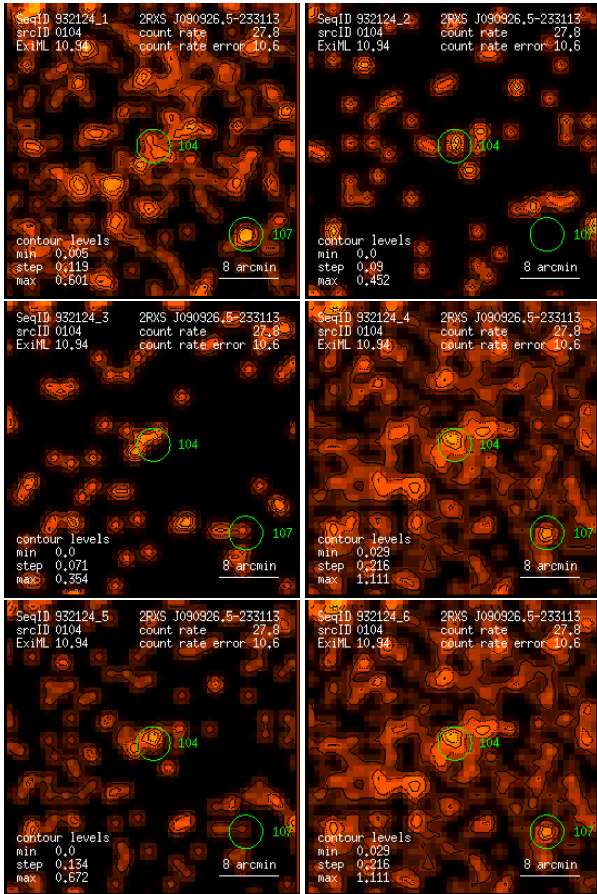
Figure 104: RASS 932124: detection 0104: band rate images, Gaussian filter: (1) PSPC channels 11 – 41, (2) 52 – 90, (3) 91 – 201, (4) 11 – 235, (5) 52 – 201, (6) 11 – 201. Broad band rates in counts/ks. Band rate contour levels in counts/ks/arcmin 2 .
