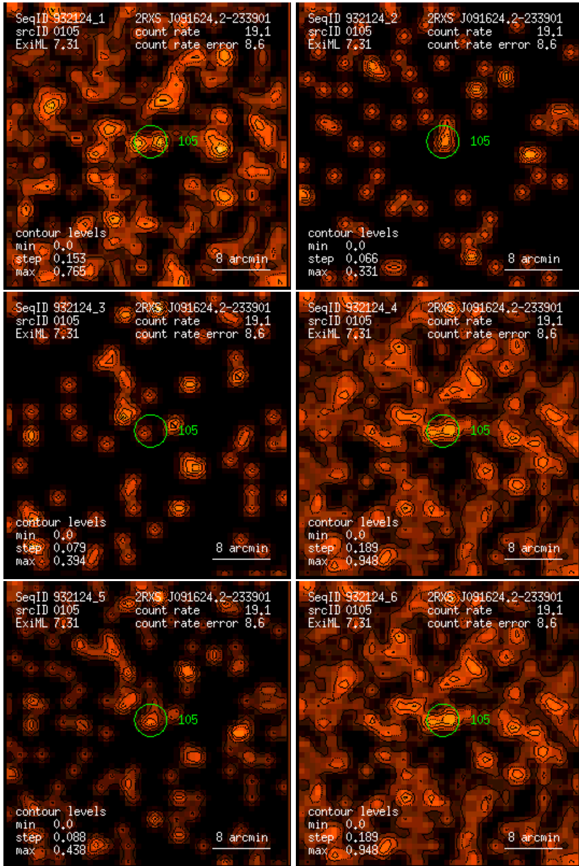
Figure 105: RASS 932124: detection 0105: band rate images, Gaussian filter: (1) PSPC channels 11 – 41, (2) 52 – 90, (3) 91 – 201, (4) 11 – 235, (5) 52 – 201, (6) 11 – 201. Broad band rates in counts/ks. Band rate contour levels in counts/ks/arcmin 2 .
