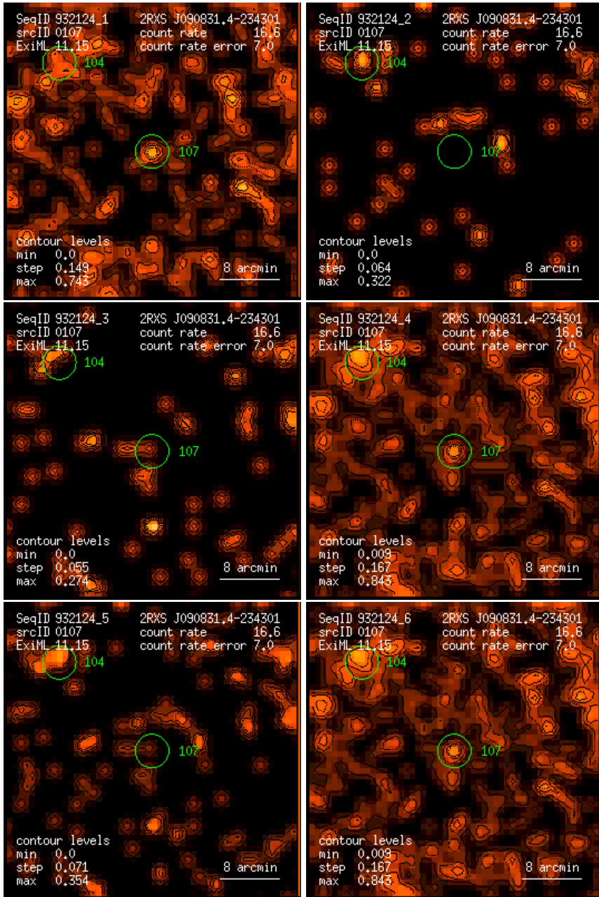
Figure 107: RASS 932124: detection 0107: band rate images, Gaussian filter: (1) PSPC channels 11 – 41, (2) 52 – 90, (3) 91 – 201, (4) 11 – 235, (5) 52 – 201, (6) 11 – 201. Broad band rates in counts/ks. Band rate contour levels in counts/ks/arcmin 2 .
