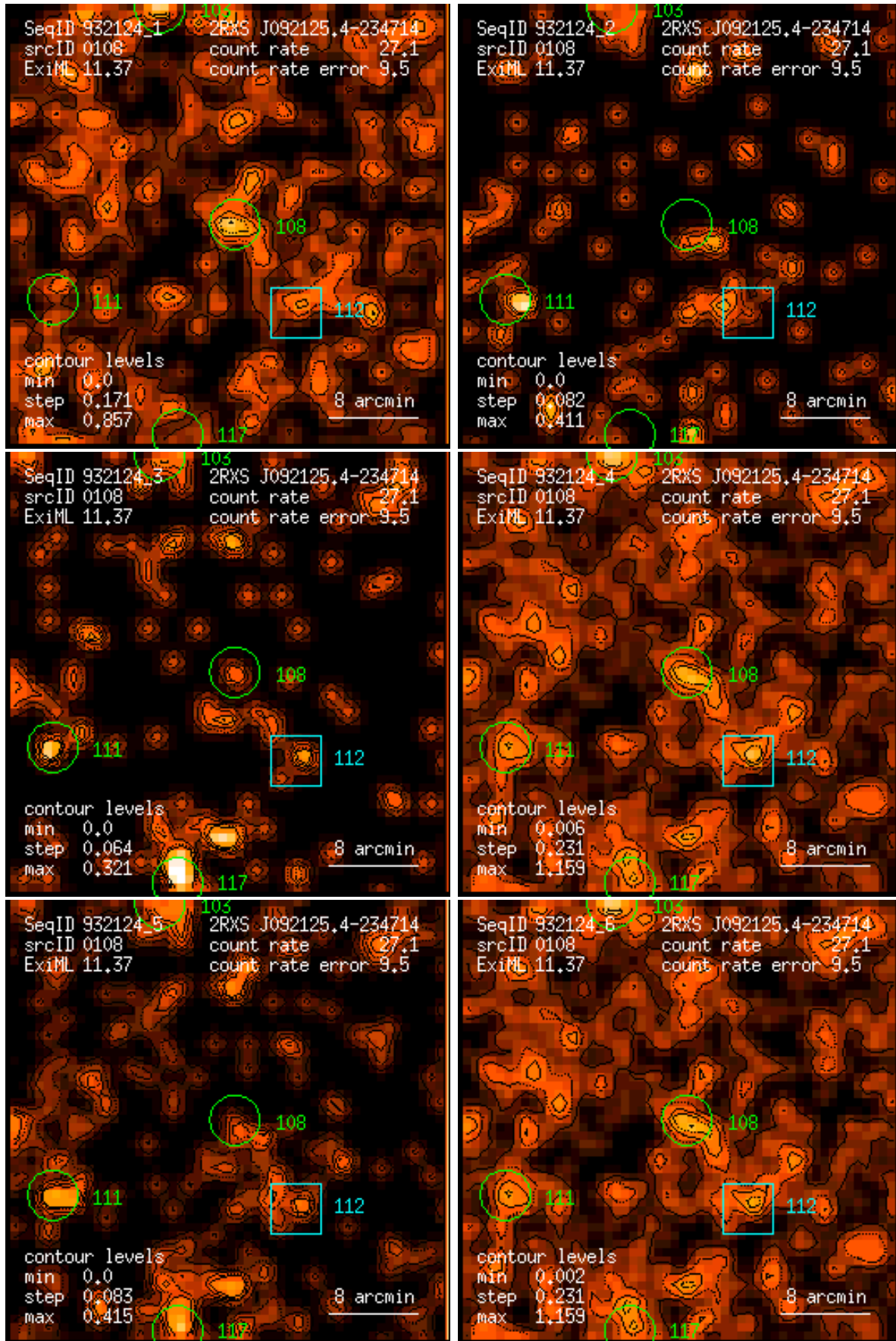
Figure 108: RASS 932124: detection 0108: band rate images, Gaussian filter: (1) PSPC channels 11 – 41, (2) 52 – 90, (3) 91 – 201, (4) 11 – 235, (5) 52 – 201, (6) 11 – 201. Broad band rates in counts/ks. Band rate contour levels in counts/ks/arcmin 2 .
