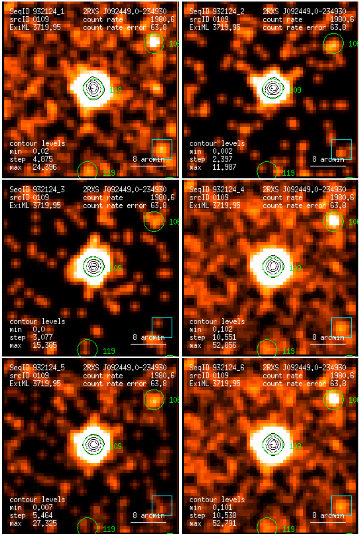
Figure 109: RASS 932124: detection 0109: band rate images, Gaussian filter: (1) PSPC channels 11 – 41, (2) 52 – 90, (3) 91 – 201, (4) 11 – 235, (5) 52 – 201, (6) 11 – 201. Broad band rates in counts/ks. Band rate contour levels in counts/ks/arcmin 2 .
