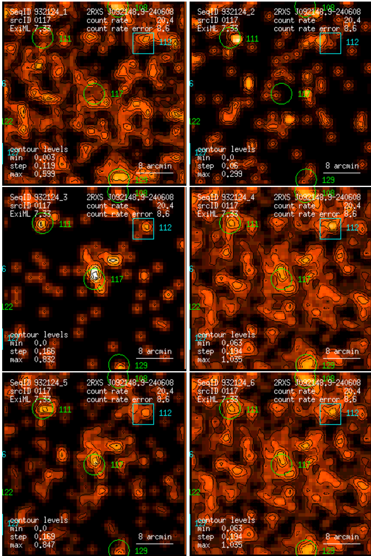
Figure 117: RASS 932124: detection 0117: band rate images, Gaussian filter: (1) PSPC channels 11 – 41, (2) 52 – 90, (3) 91 – 201, (4) 11 – 235, (5) 52 – 201, (6) 11 – 201. Broad band rates in counts/ks. Band rate contour levels in counts/ks/arcmin 2 .
