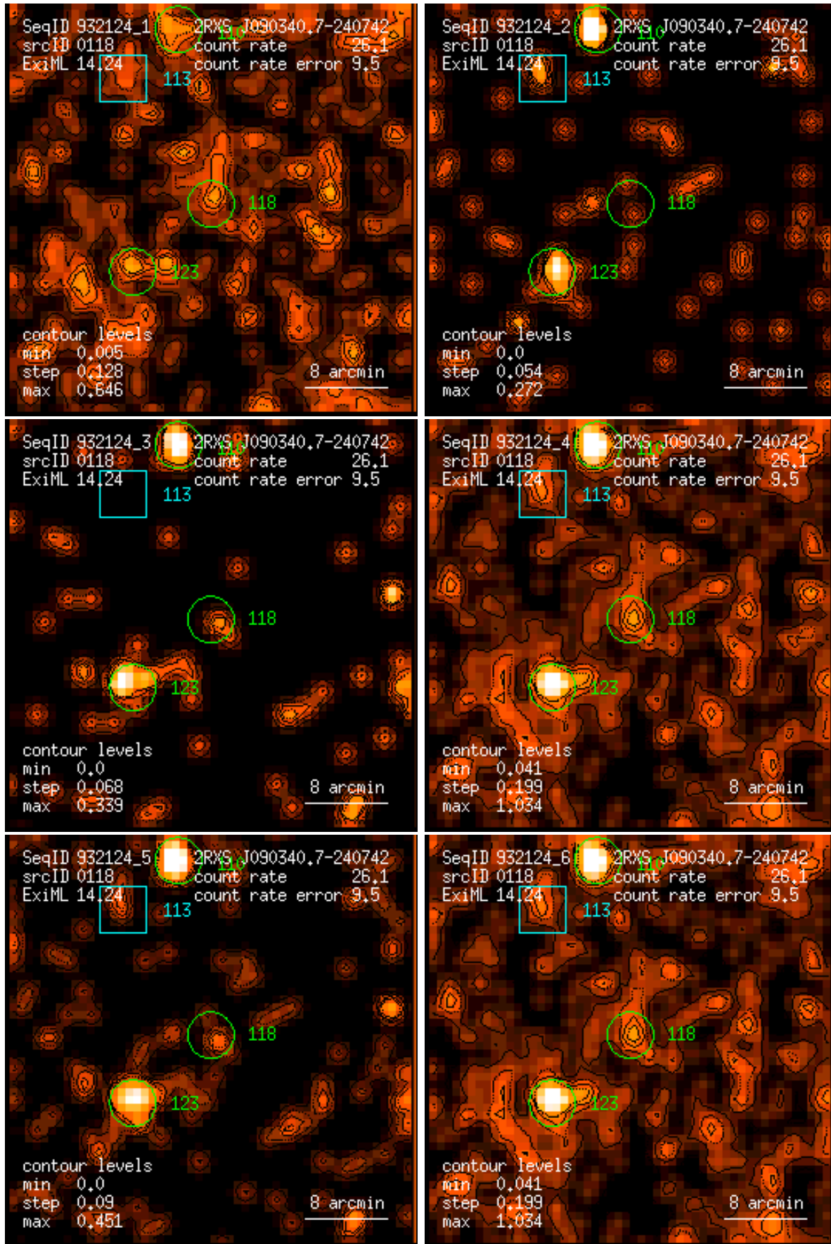
Figure 118: RASS 932124: detection 0118: band rate images, Gaussian filter: (1) PSPC channels 11 – 41, (2) 52 – 90, (3) 91 – 201, (4) 11 – 235, (5) 52 – 201, (6) 11 – 201. Broad band rates in counts/ks. Band rate contour levels in counts/ks/arcmin 2 .
