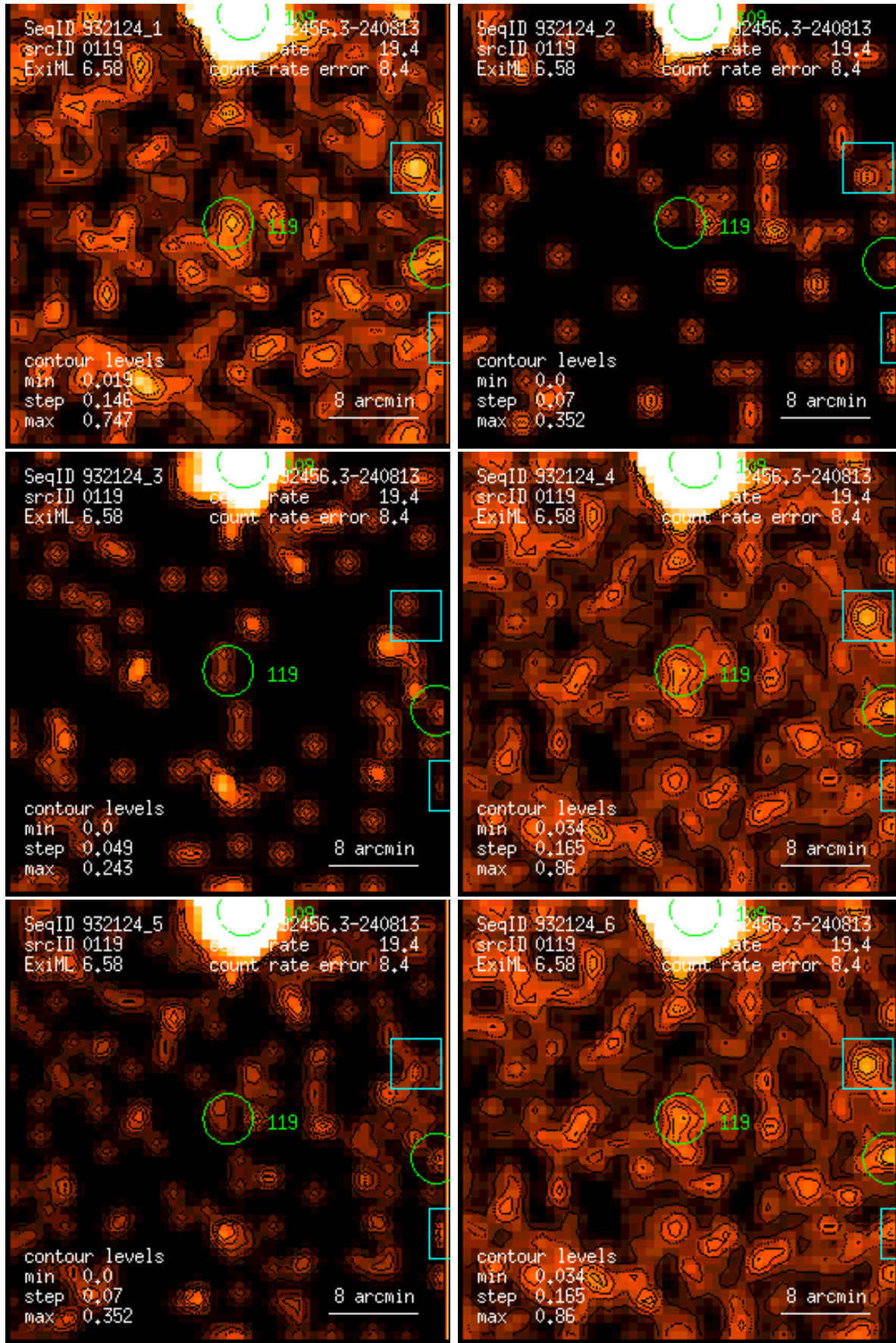
Figure 119: RASS 932124: detection 0119: band rate images, Gaussian filter: (1) PSPC channels 11 – 41, (2) 52 – 90, (3) 91 – 201, (4) 11 – 235, (5) 52 – 201, (6) 11 – 201. Broad band rates in counts/ks. Band rate contour levels in counts/ks/arcmin 2 .
