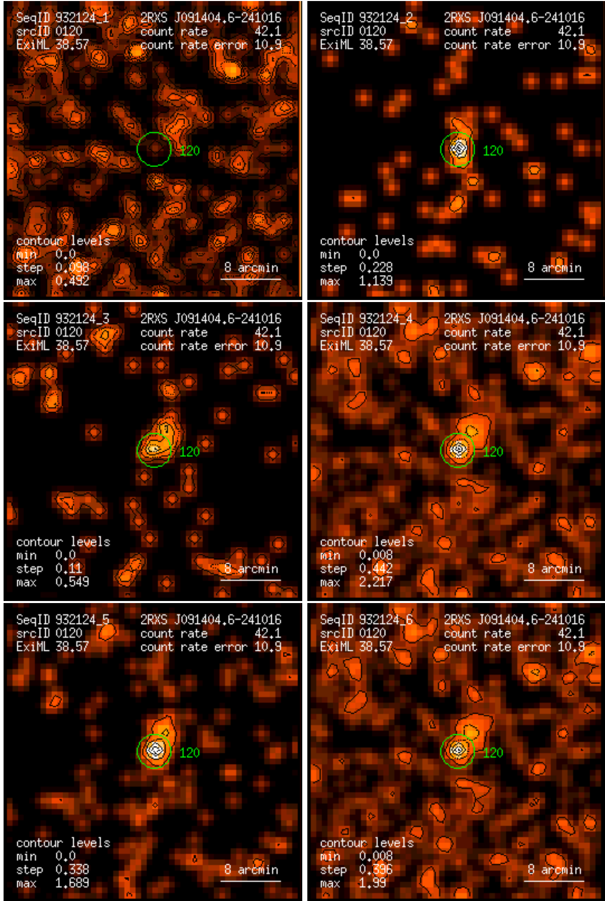
Figure 120: RASS 932124: detection 0120: band rate images, Gaussian filter: (1) PSPC channels 11 – 41, (2) 52 – 90, (3) 91 – 201, (4) 11 – 235, (5) 52 – 201, (6) 11 – 201. Broad band rates in counts/ks. Band rate contour levels in counts/ks/arcmin 2 .
