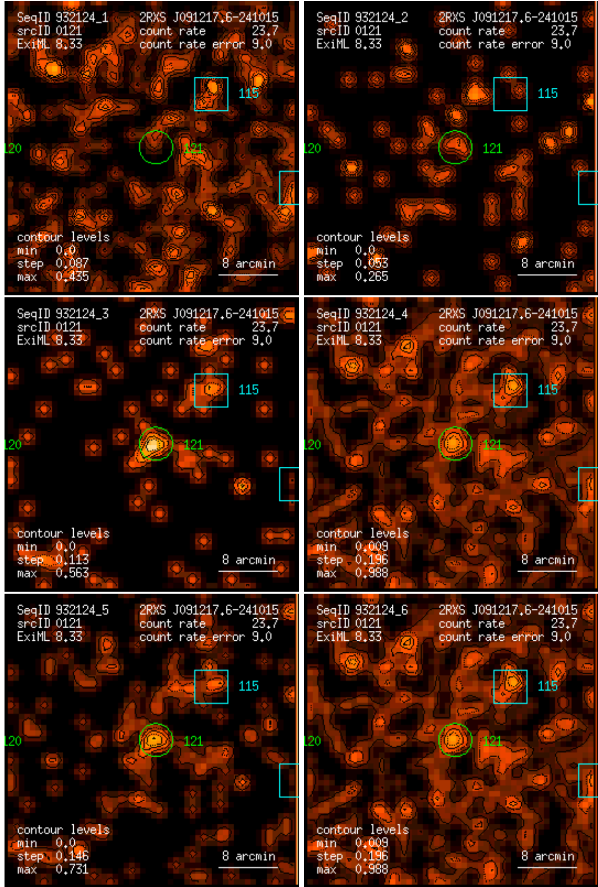
Figure 121: RASS 932124: detection 0121: band rate images, Gaussian filter: (1) PSPC channels 11 – 41, (2) 52 – 90, (3) 91 – 201, (4) 11 – 235, (5) 52 – 201, (6) 11 – 201. Broad band rates in counts/ks. Band rate contour levels in counts/ks/arcmin 2 .
