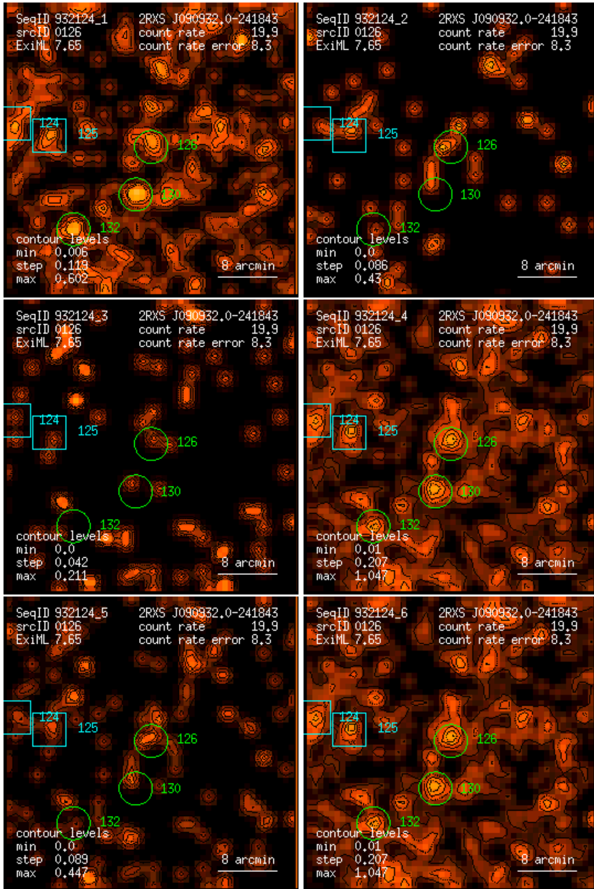
Figure 126: RASS 932124: detection 0126: band rate images, Gaussian filter: (1) PSPC channels 11 – 41, (2) 52 – 90, (3) 91 – 201, (4) 11 – 235, (5) 52 – 201, (6) 11 – 201. Broad band rates in counts/ks. Band rate contour levels in counts/ks/arcmin 2 .
