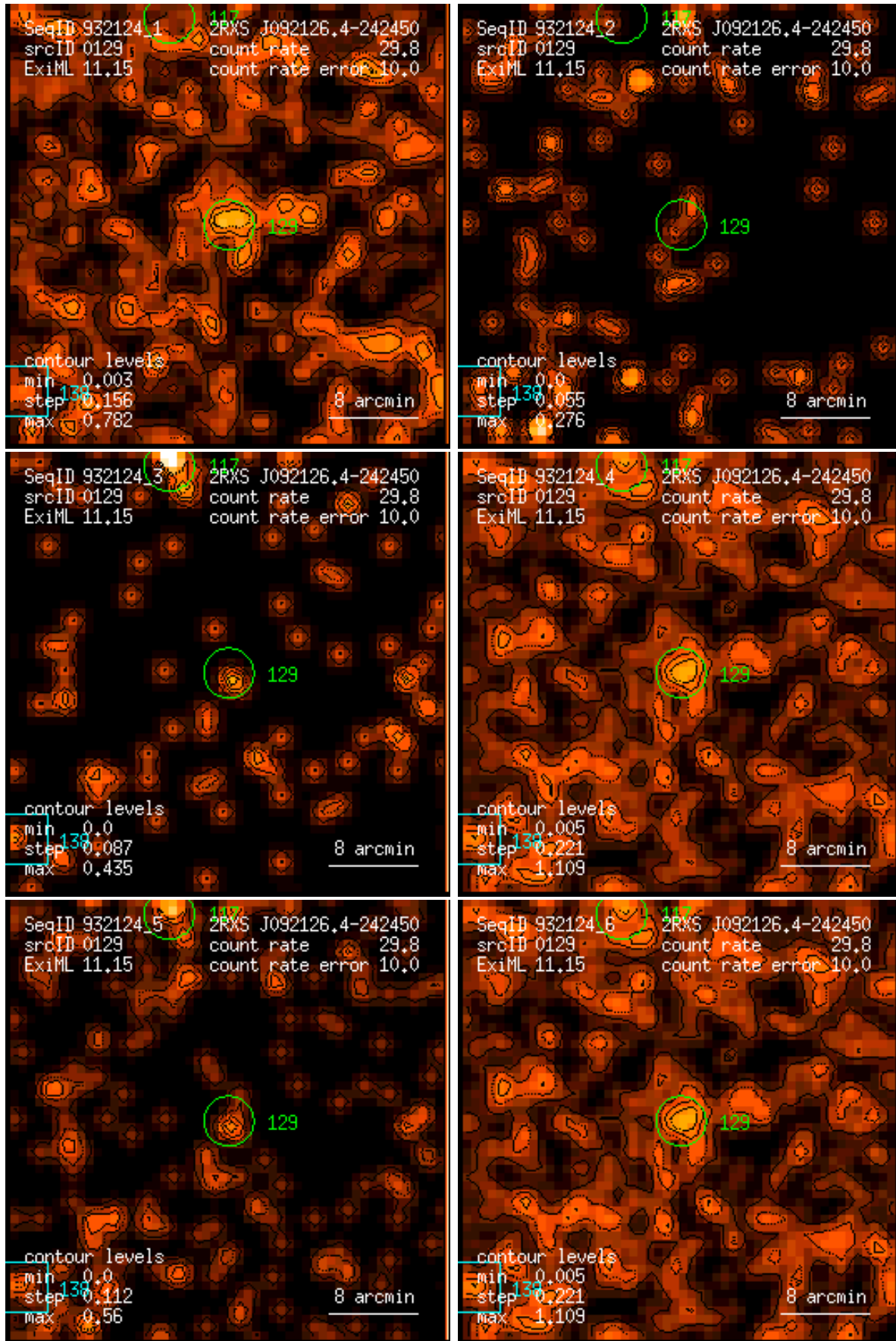
Figure 129: RASS 932124: detection 0129: band rate images, Gaussian filter: (1) PSPC channels 11 – 41, (2) 52 – 90, (3) 91 – 201, (4) 11 – 235, (5) 52 – 201, (6) 11 – 201. Broad band rates in counts/ks. Band rate contour levels in counts/ks/arcmin 2 .
