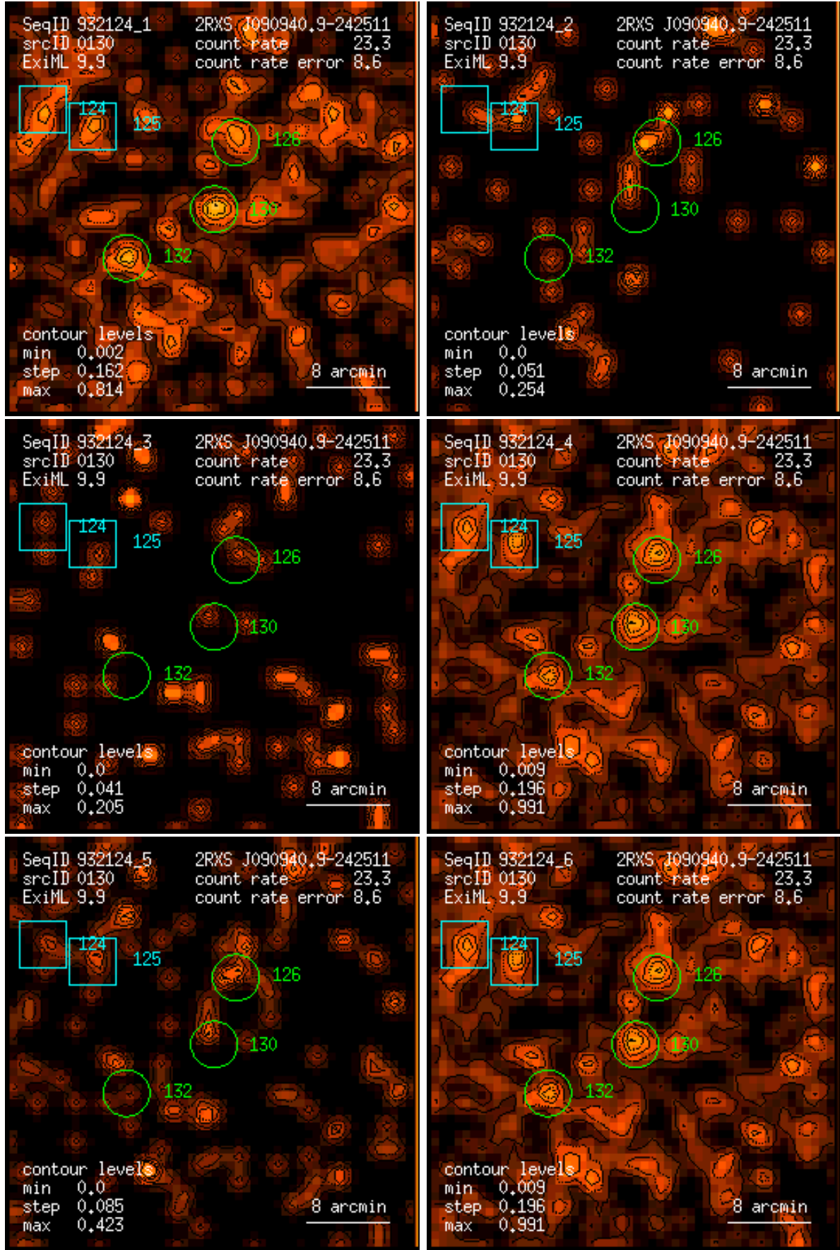
Figure 130: RASS 932124: detection 0130: band rate images, Gaussian filter: (1) PSPC channels 11 – 41, (2) 52 – 90, (3) 91 – 201, (4) 11 – 235, (5) 52 – 201, (6) 11 – 201. Broad band rates in counts/ks. Band rate contour levels in counts/ks/arcmin 2 .
