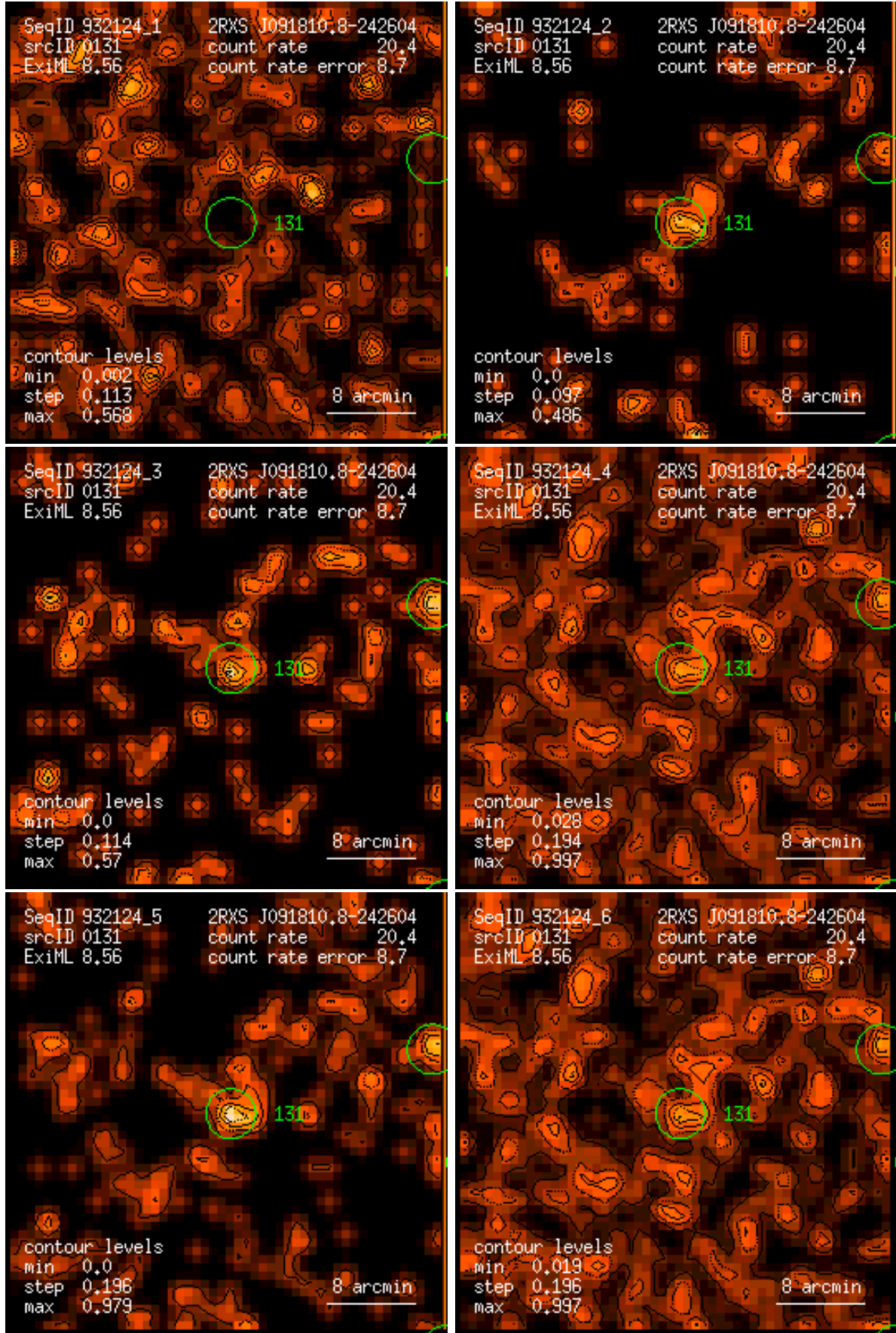
Figure 131: RASS 932124: detection 0131: band rate images, Gaussian filter: (1) PSPC channels 11 – 41, (2) 52 – 90, (3) 91 – 201, (4) 11 – 235, (5) 52 – 201, (6) 11 – 201. Broad band rates in counts/ks. Band rate contour levels in counts/ks/arcmin 2 .
