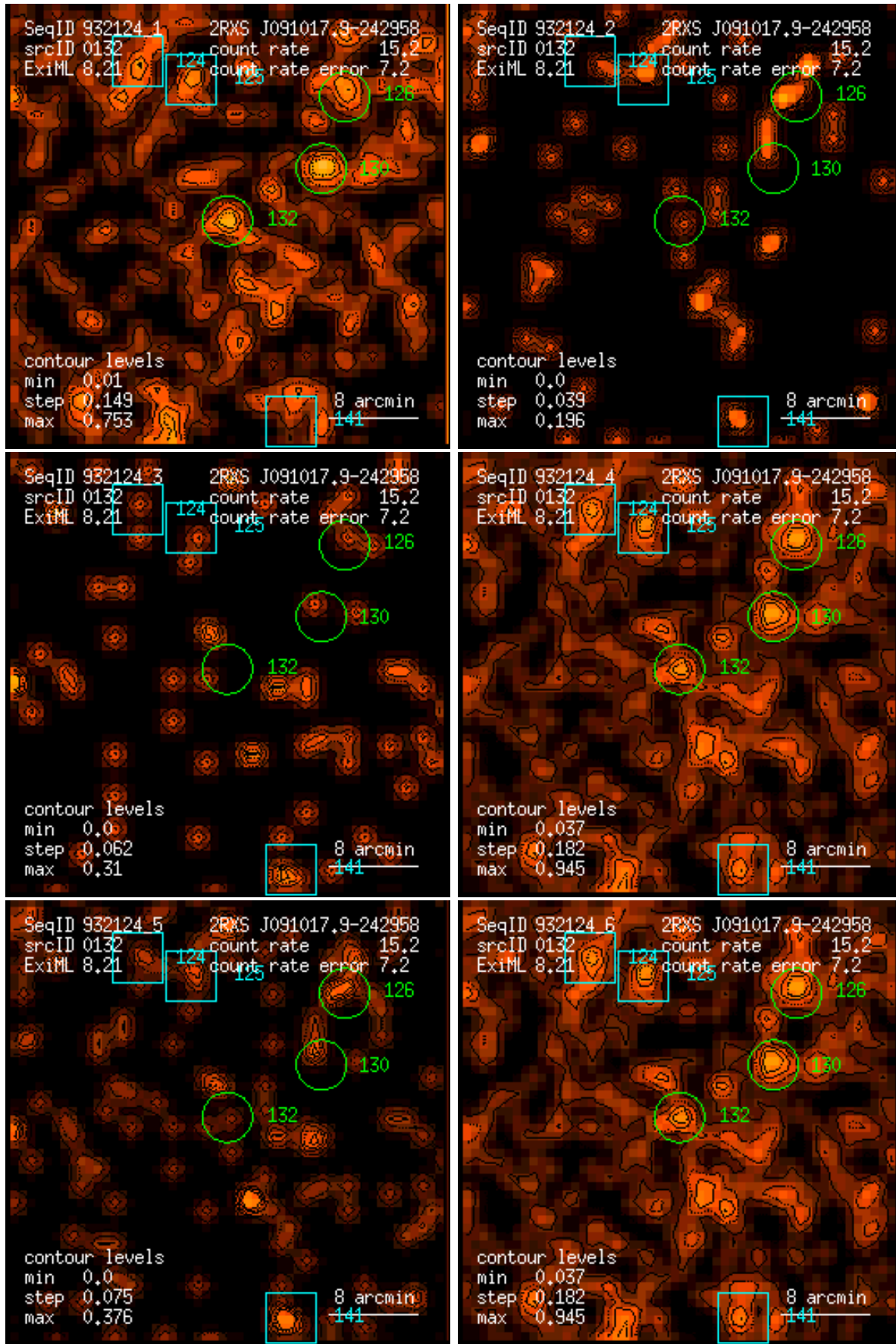
Figure 132: RASS 932124: detection 0132: band rate images, Gaussian filter: (1) PSPC channels 11 – 41, (2) 52 – 90, (3) 91 – 201, (4) 11 – 235, (5) 52 – 201, (6) 11 – 201. Broad band rates in counts/ks. Band rate contour levels in counts/ks/arcmin 2 .
