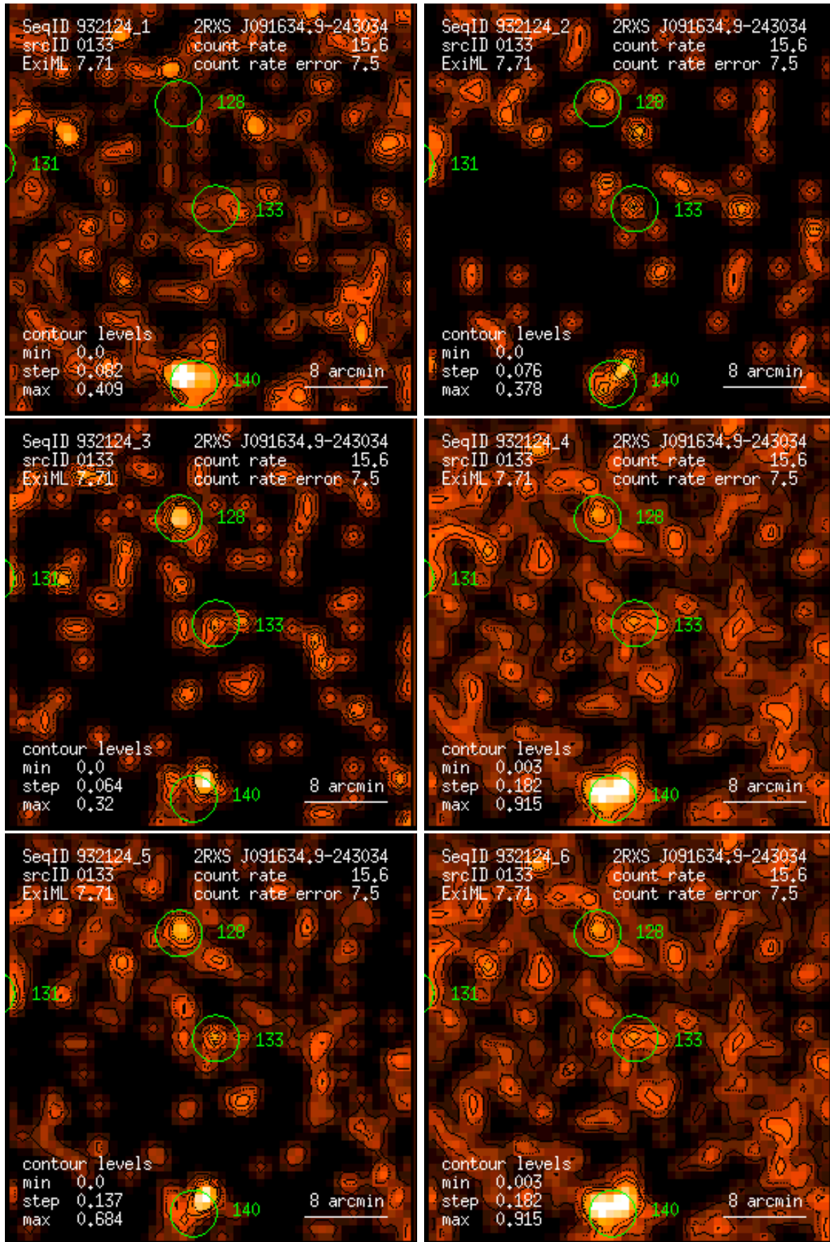
Figure 133: RASS 932124: detection 0133: band rate images, Gaussian filter: (1) PSPC channels 11 – 41, (2) 52 – 90, (3) 91 – 201, (4) 11 – 235, (5) 52 – 201, (6) 11 – 201. Broad band rates in counts/ks. Band rate contour levels in counts/ks/arcmin 2 .
