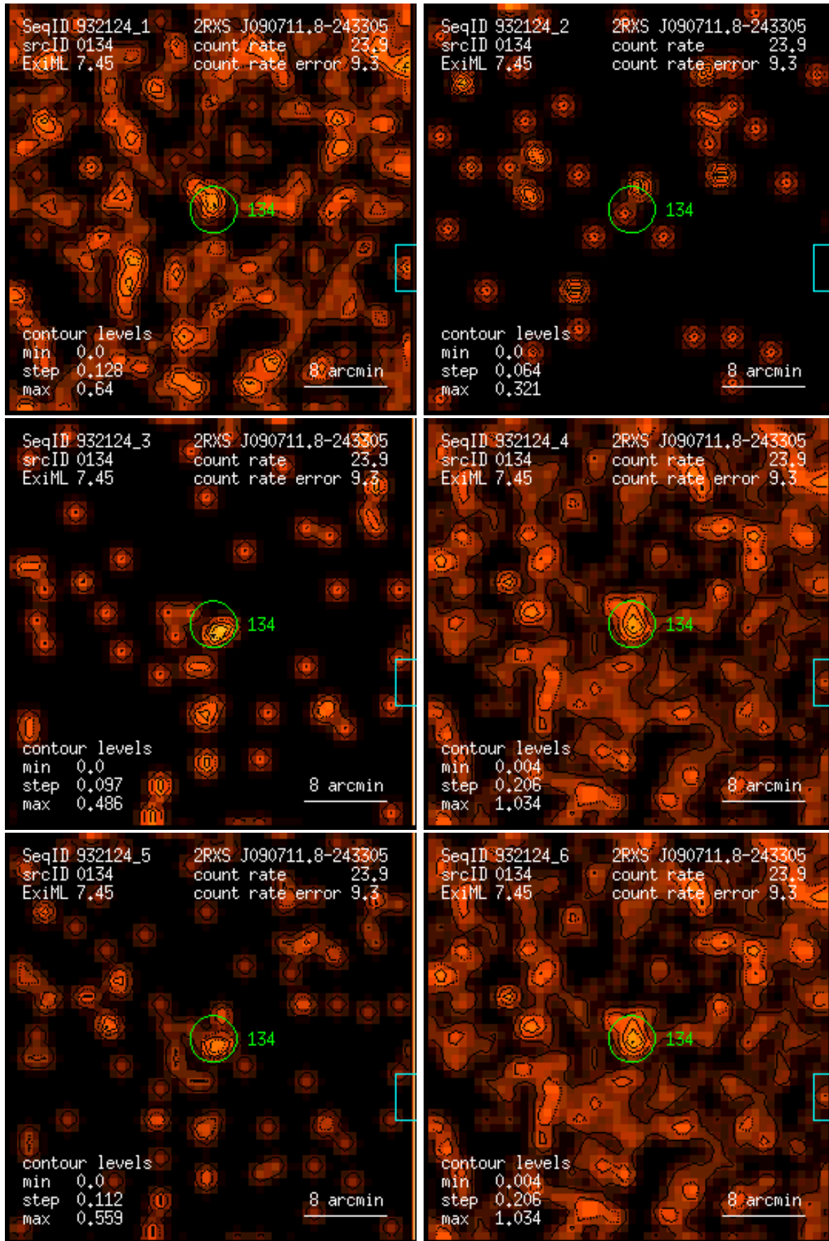
Figure 134: RASS 932124: detection 0134: band rate images, Gaussian filter: (1) PSPC channels 11 – 41, (2) 52 – 90, (3) 91 – 201, (4) 11 – 235, (5) 52 – 201, (6) 11 – 201. Broad band rates in counts/ks. Band rate contour levels in counts/ks/arcmin 2 .
