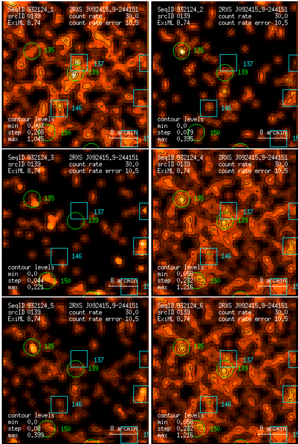
Figure 139: RASS 932124: detection 0139: band rate images, Gaussian filter: (1) PSPC channels 11 – 41, (2) 52 – 90, (3) 91 – 201, (4) 11 – 235, (5) 52 – 201, (6) 11 – 201. Broad band rates in counts/ks. Band rate contour levels in counts/ks/arcmin 2 .
