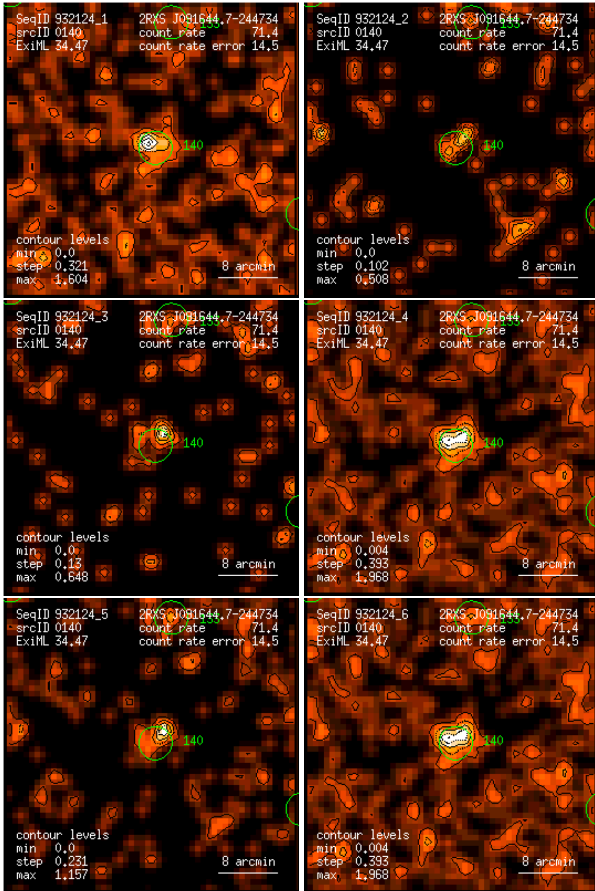
Figure 140: RASS 932124: detection 0140: band rate images, Gaussian filter: (1) PSPC channels 11 – 41, (2) 52 – 90, (3) 91 – 201, (4) 11 – 235, (5) 52 – 201, (6) 11 – 201. Broad band rates in counts/ks. Band rate contour levels in counts/ks/arcmin 2 .
