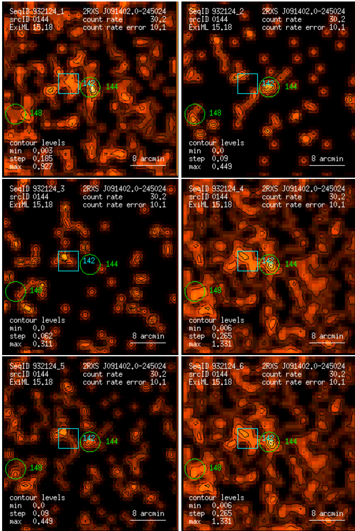
Figure 144: RASS 932124: detection 0144: band rate images, Gaussian filter: (1) PSPC channels 11 – 41, (2) 52 – 90, (3) 91 – 201, (4) 11 – 235, (5) 52 – 201, (6) 11 – 201. Broad band rates in counts/ks. Band rate contour levels in counts/ks/arcmin 2 .
