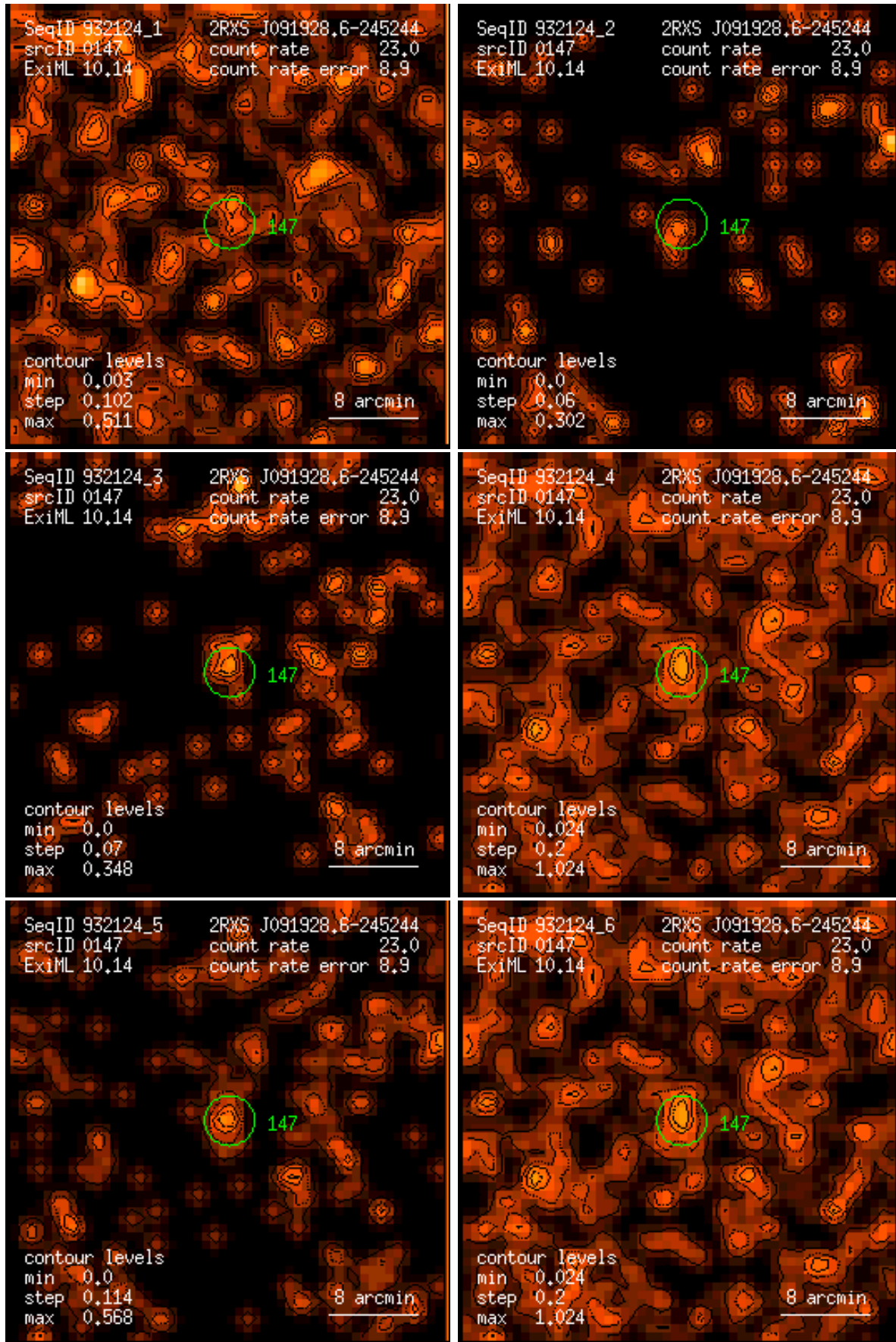
Figure 147: RASS 932124: detection 0147: band rate images, Gaussian filter: (1) PSPC channels 11 – 41, (2) 52 – 90, (3) 91 – 201, (4) 11 – 235, (5) 52 – 201, (6) 11 – 201. Broad band rates in counts/ks. Band rate contour levels in counts/ks/arcmin 2 .
