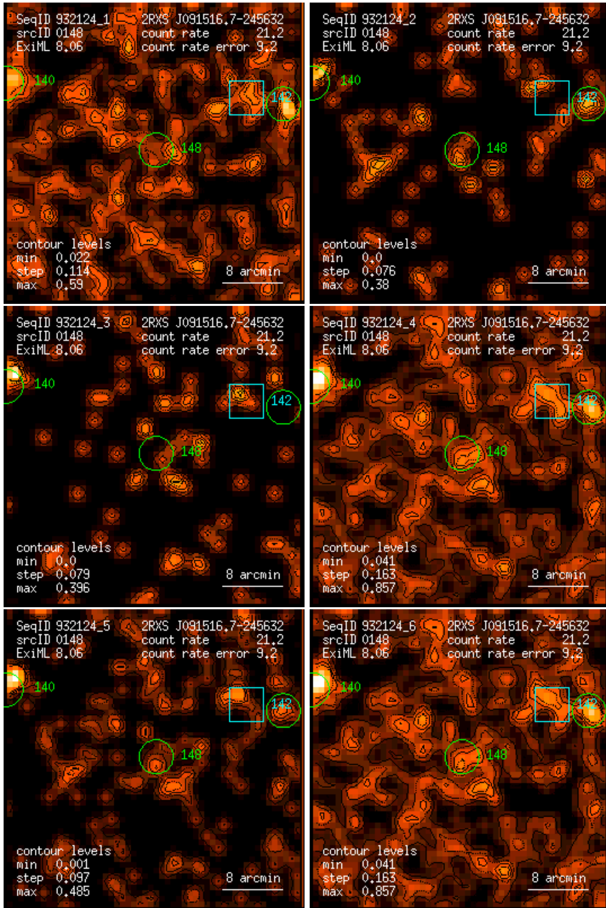
Figure 148: RASS 932124: detection 0148: band rate images, Gaussian filter: (1) PSPC channels 11 – 41, (2) 52 – 90, (3) 91 – 201, (4) 11 – 235, (5) 52 – 201, (6) 11 – 201. Broad band rates in counts/ks. Band rate contour levels in counts/ks/arcmin 2 .
