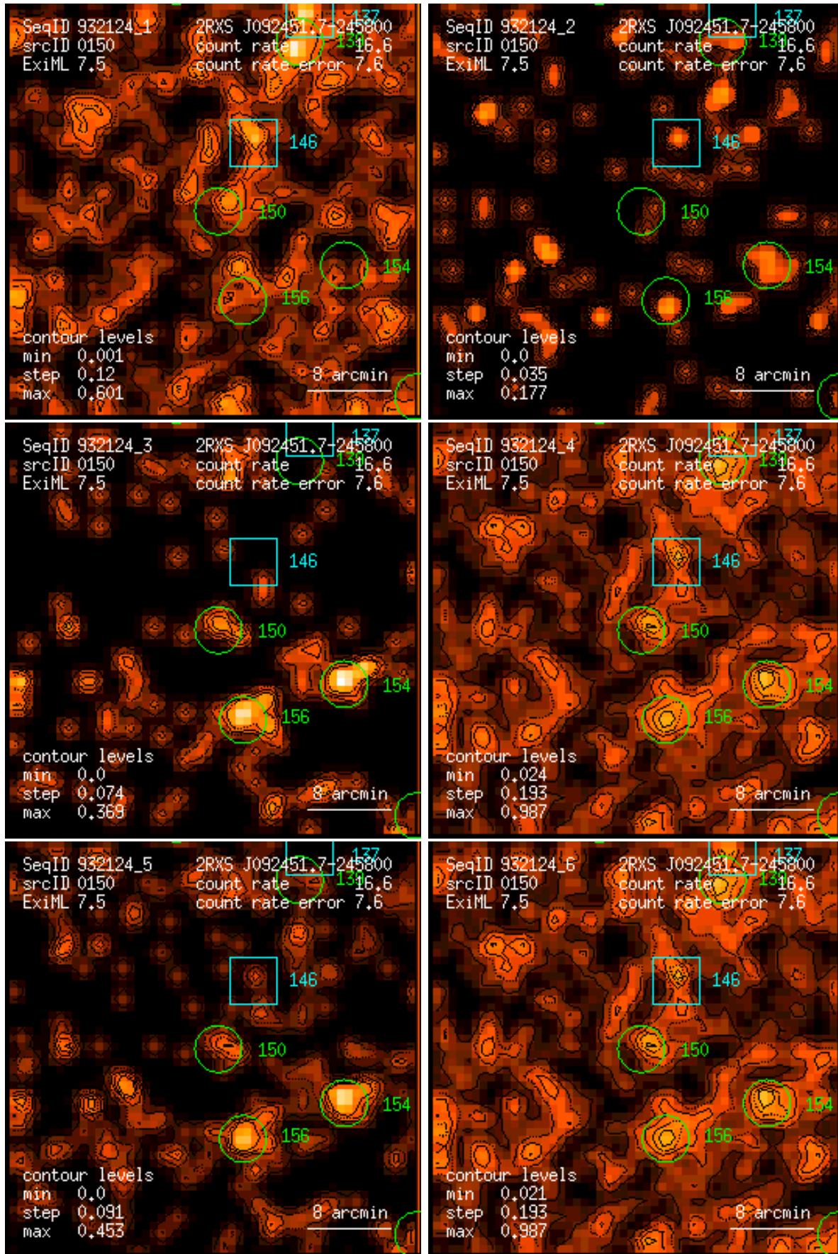
Figure 150: RASS 932124: detection 0150: band rate images, Gaussian filter: (1) PSPC channels 11 – 41, (2) 52 – 90, (3) 91 – 201, (4) 11 – 235, (5) 52 – 201, (6) 11 – 201. Broad band rates in counts/ks. Band rate contour levels in counts/ks/arcmin 2 .
