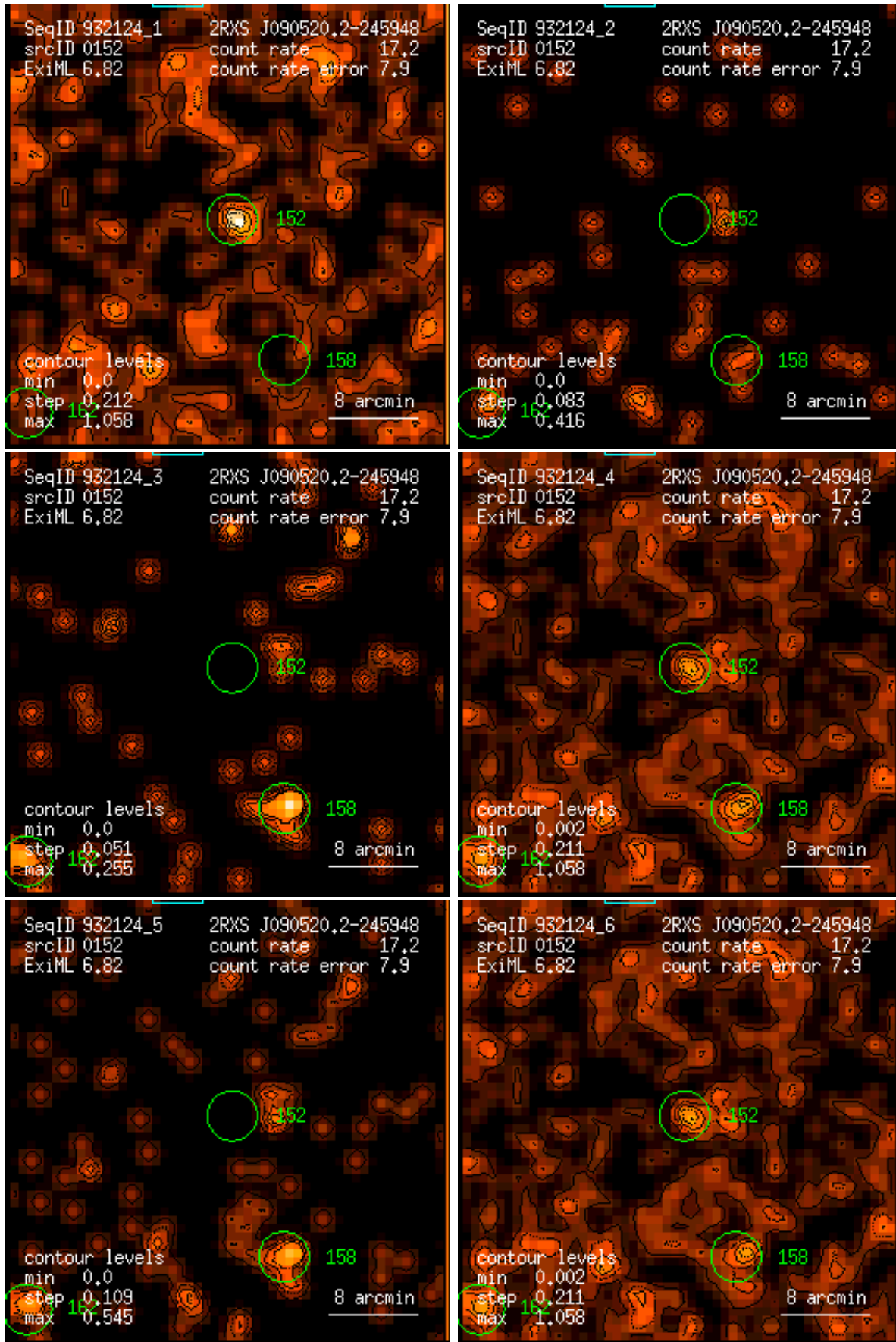
Figure 152: RASS 932124: detection 0152: band rate images, Gaussian filter: (1) PSPC channels 11 – 41, (2) 52 – 90, (3) 91 – 201, (4) 11 – 235, (5) 52 – 201, (6) 11 – 201. Broad band rates in counts/ks. Band rate contour levels in counts/ks/arcmin 2 .
