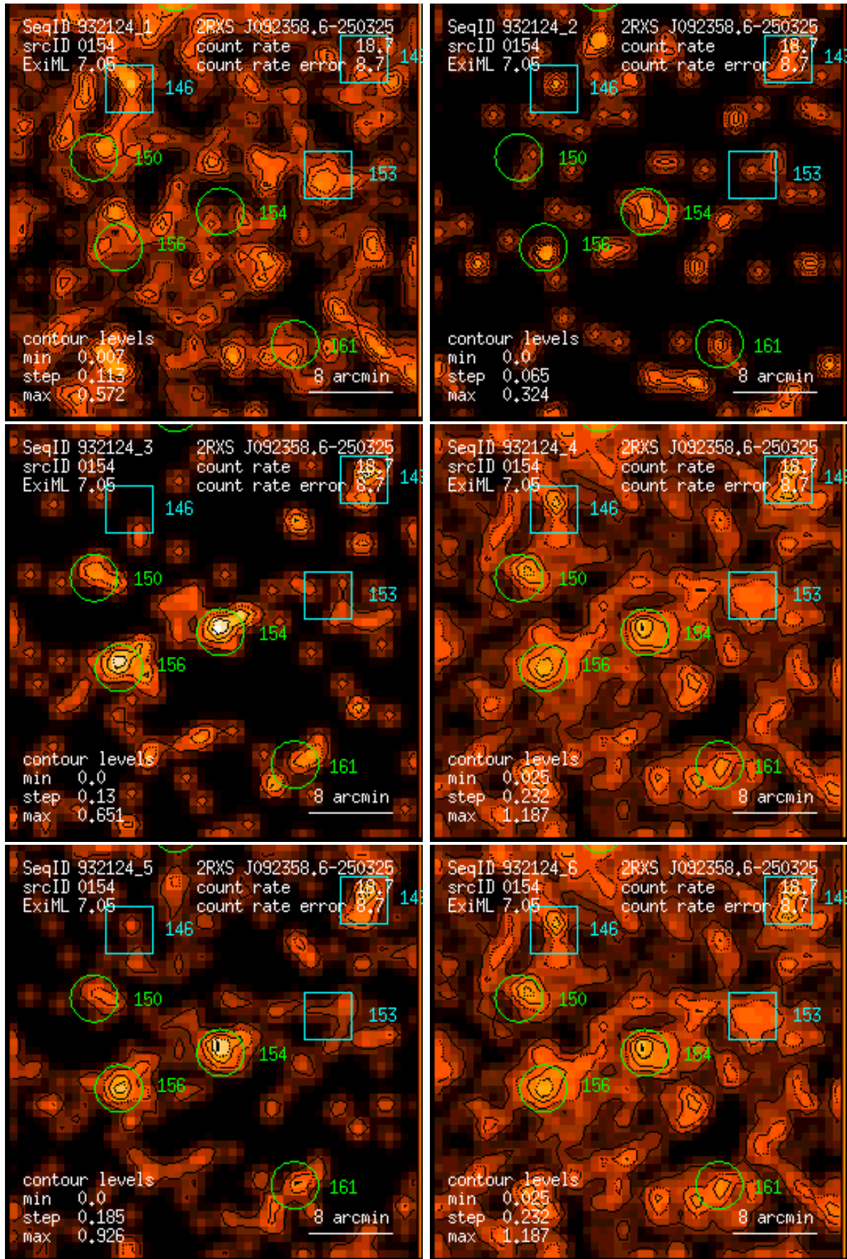
Figure 154: RASS 932124: detection 0154: band rate images, Gaussian filter: (1) PSPC channels 11 – 41, (2) 52 – 90, (3) 91 – 201, (4) 11 – 235, (5) 52 – 201, (6) 11 – 201. Broad band rates in counts/ks. Band rate contour levels in counts/ks/arcmin 2 .
