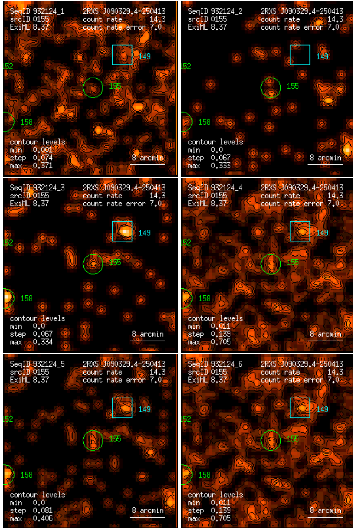
Figure 155: RASS 932124: detection 0155: band rate images, Gaussian filter: (1) PSPC channels 11 – 41, (2) 52 – 90, (3) 91 – 201, (4) 11 – 235, (5) 52 – 201, (6) 11 – 201. Broad band rates in counts/ks. Band rate contour levels in counts/ks/arcmin 2 .
