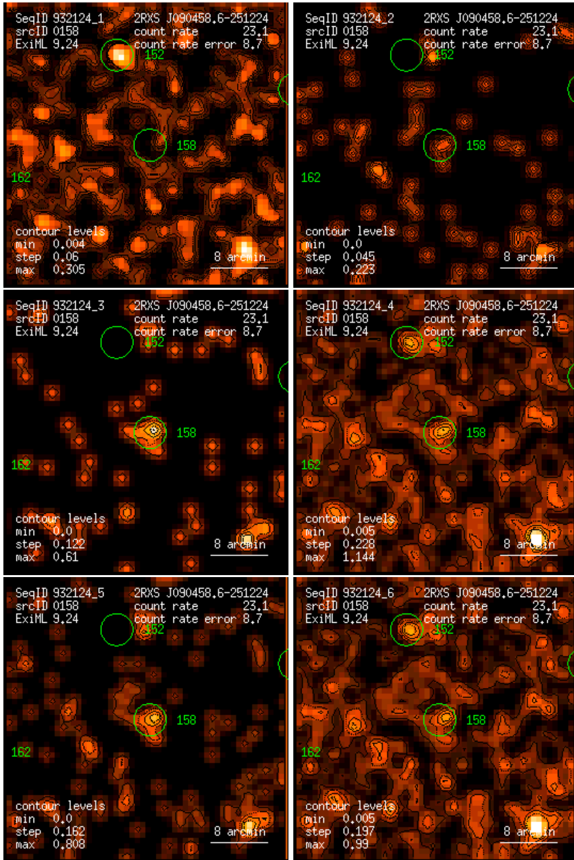
Figure 158: RASS 932124: detection 0158: band rate images, Gaussian filter: (1) PSPC channels 11 – 41, (2) 52 – 90, (3) 91 – 201, (4) 11 – 235, (5) 52 – 201, (6) 11 – 201. Broad band rates in counts/ks. Band rate contour levels in counts/ks/arcmin 2 .
