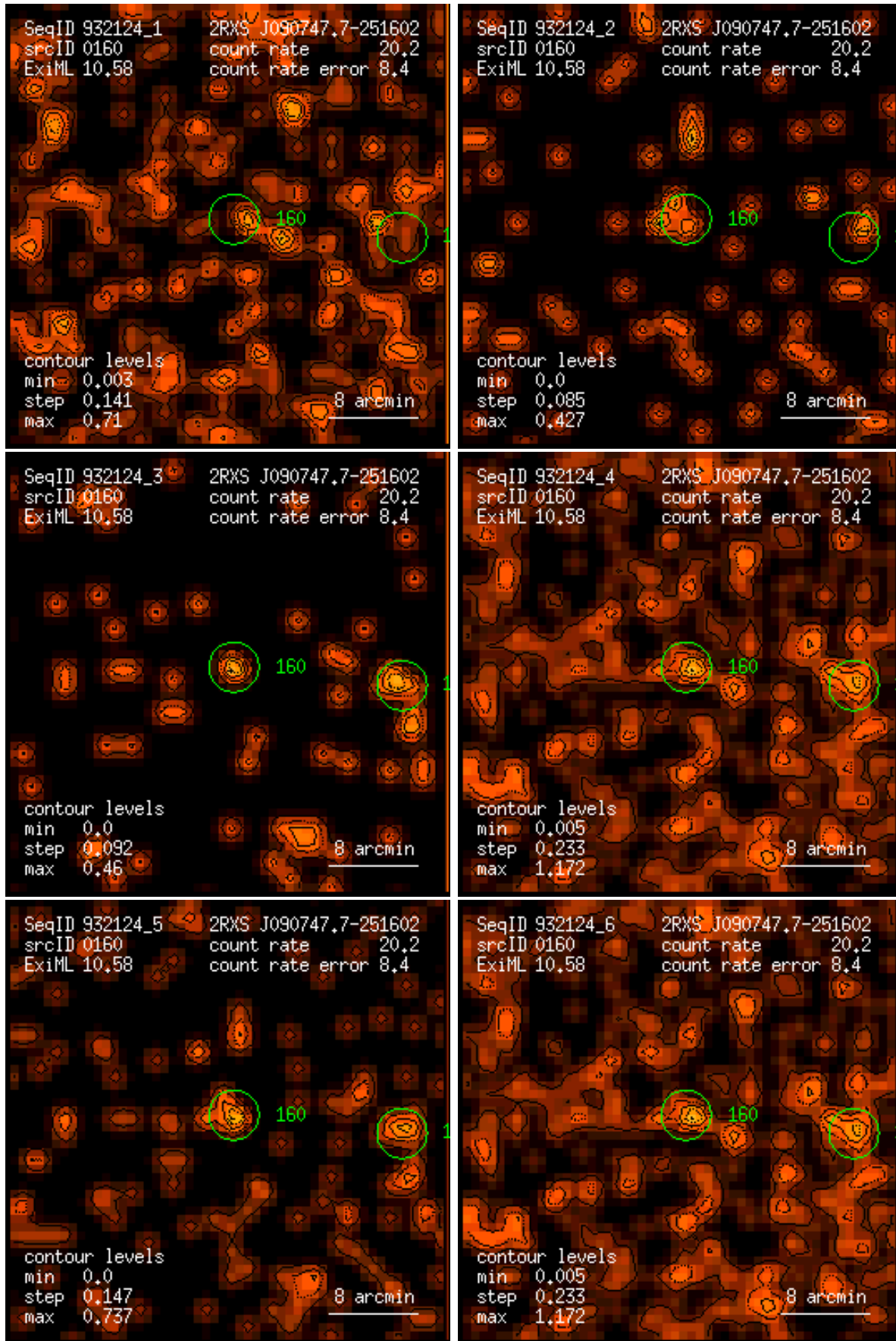
Figure 160: RASS 932124: detection 0160: band rate images, Gaussian filter: (1) PSPC channels 11 – 41, (2) 52 – 90, (3) 91 – 201, (4) 11 – 235, (5) 52 – 201, (6) 11 – 201. Broad band rates in counts/ks. Band rate contour levels in counts/ks/arcmin 2 .
