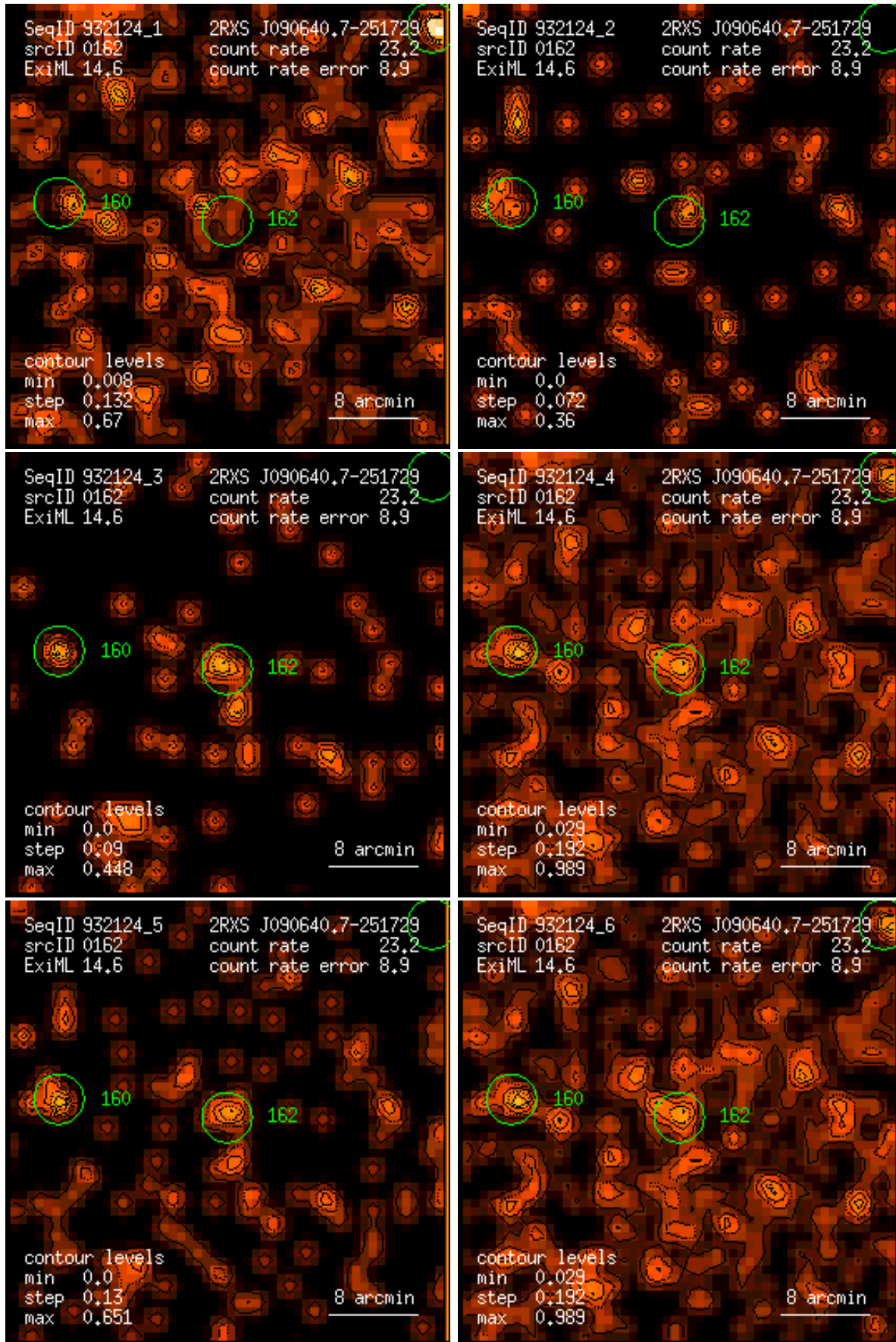
Figure 162: RASS 932124: detection 0162: band rate images, Gaussian filter: (1) PSPC channels 11 – 41, (2) 52 – 90, (3) 91 – 201, (4) 11 – 235, (5) 52 – 201, (6) 11 – 201. Broad band rates in counts/ks. Band rate contour levels in counts/ks/arcmin 2 .
