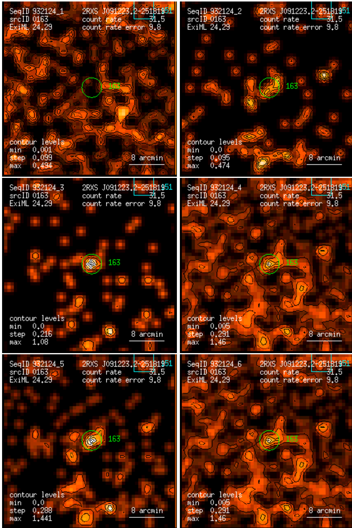
Figure 163: RASS 932124: detection 0163: band rate images, Gaussian filter: (1) PSPC channels 11 – 41, (2) 52 – 90, (3) 91 – 201, (4) 11 – 235, (5) 52 – 201, (6) 11 – 201. Broad band rates in counts/ks. Band rate contour levels in counts/ks/arcmin 2 .
