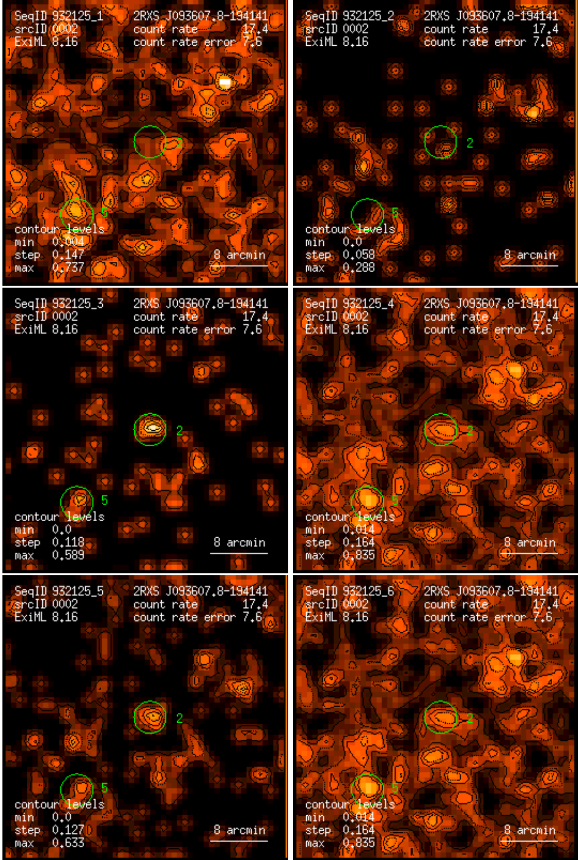
Figure 2: RASS 932125: detection 0002: band rate images, Gaussian filter: (1) PSPC channels 11 – 41, (2) 52 – 90, (3) 91 – 201, (4) 11 – 235, (5) 52 – 201, (6) 11 – 201. Broad band rates in counts/ks. Band rate contour levels in counts/ks/arcmin 2 .
