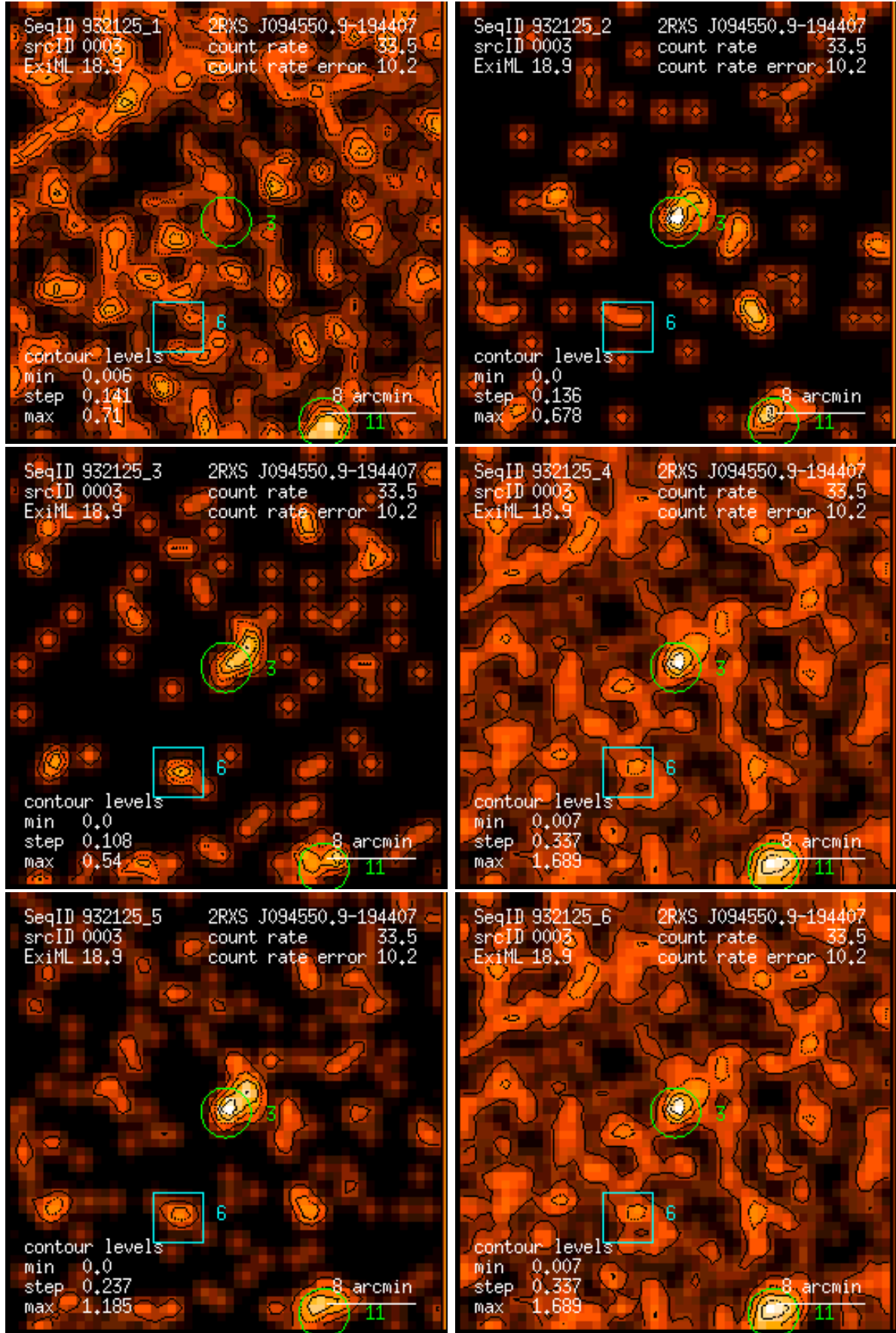
Figure 3: RASS 932125: detection 0003: band rate images, Gaussian filter: (1) PSPC channels 11 – 41, (2) 52 – 90, (3) 91 – 201, (4) 11 – 235, (5) 52 – 201, (6) 11 – 201. Broad band rates in counts/ks. Band rate contour levels in counts/ks/arcmin 2 .
