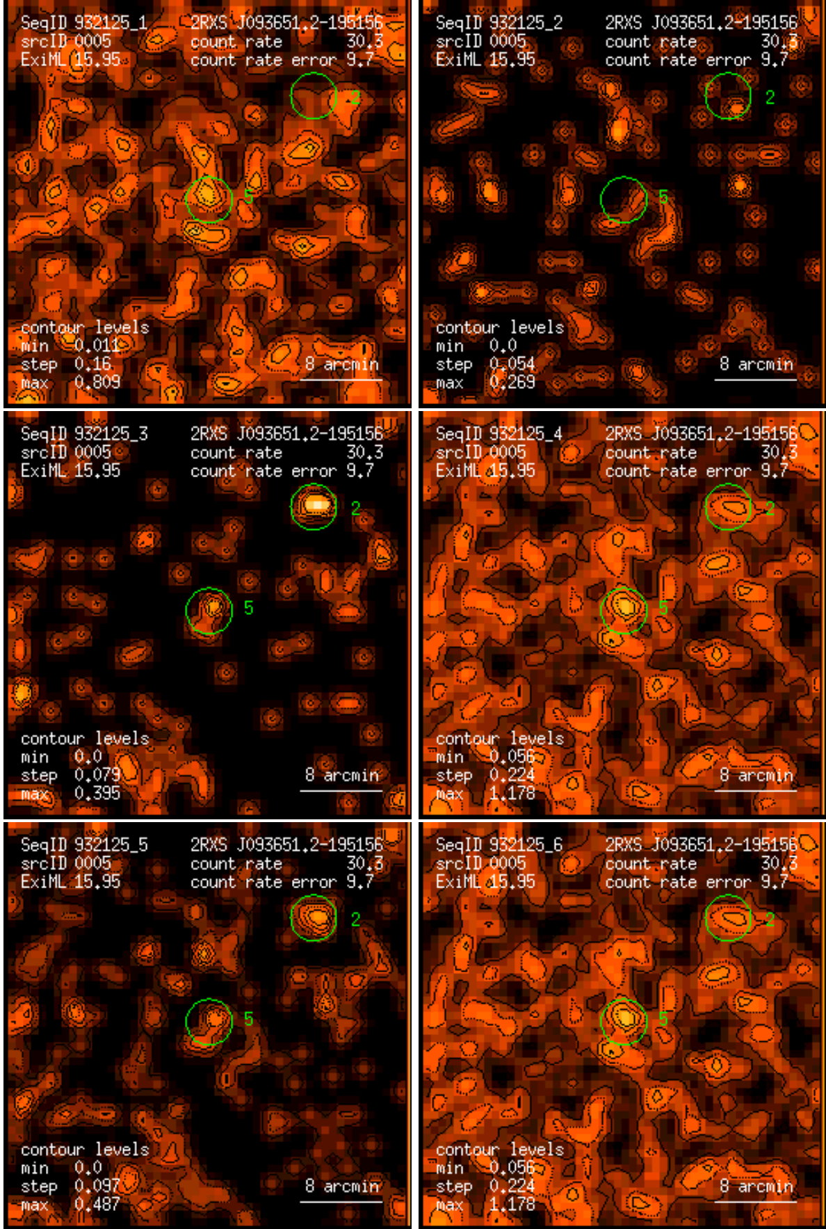
Figure 5: RASS 932125: detection 0005: band rate images, Gaussian filter: (1) PSPC channels 11 – 41, (2) 52 – 90, (3) 91 – 201, (4) 11 – 235, (5) 52 – 201, (6) 11 – 201. Broad band rates in counts/ks. Band rate contour levels in counts/ks/arcmin 2 .
