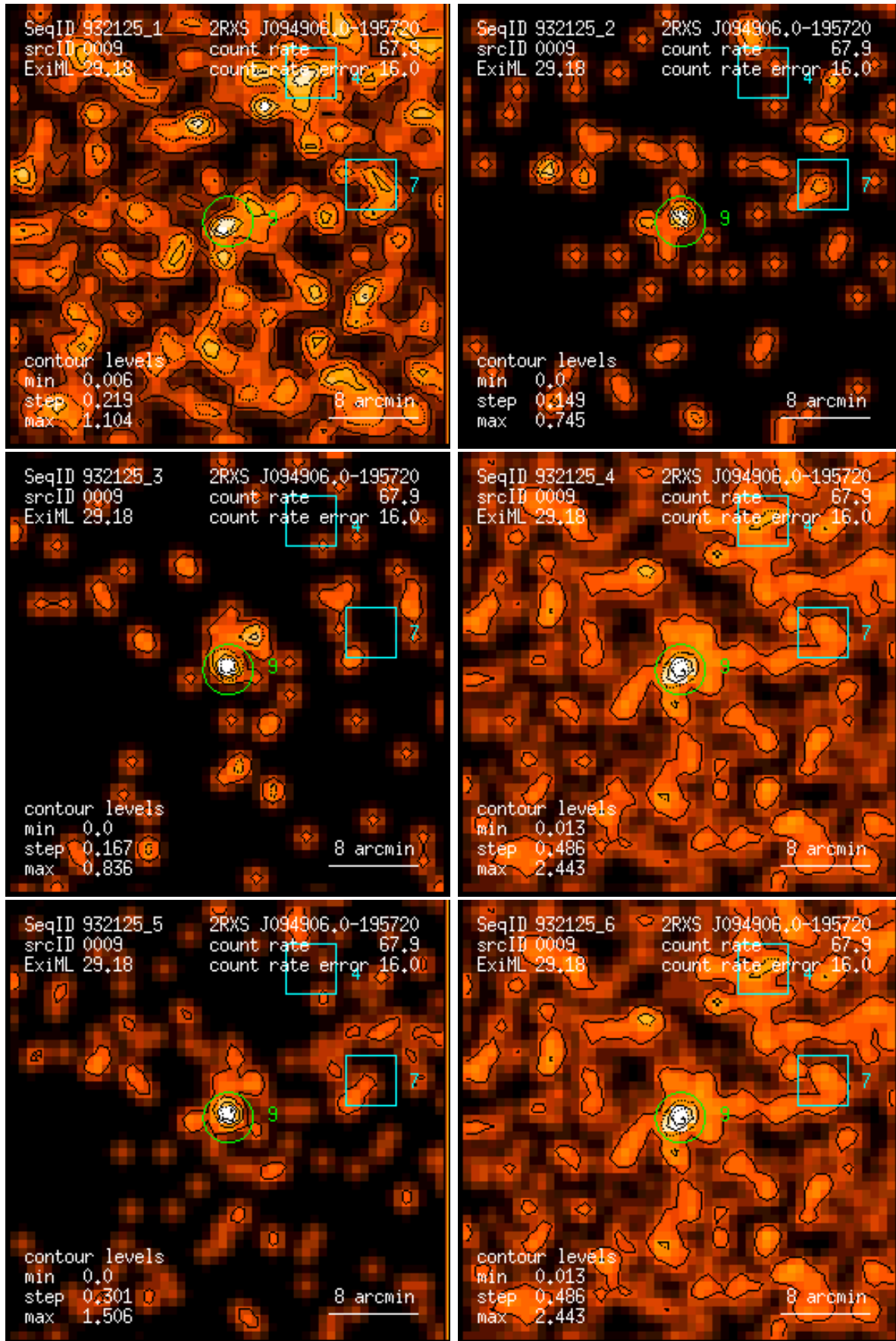
Figure 9: RASS 932125: detection 0009: band rate images, Gaussian filter: (1) PSPC channels 11 – 41, (2) 52 – 90, (3) 91 – 201, (4) 11 – 235, (5) 52 – 201, (6) 11 – 201. Broad band rates in counts/ks. Band rate contour levels in counts/ks/arcmin 2 .
