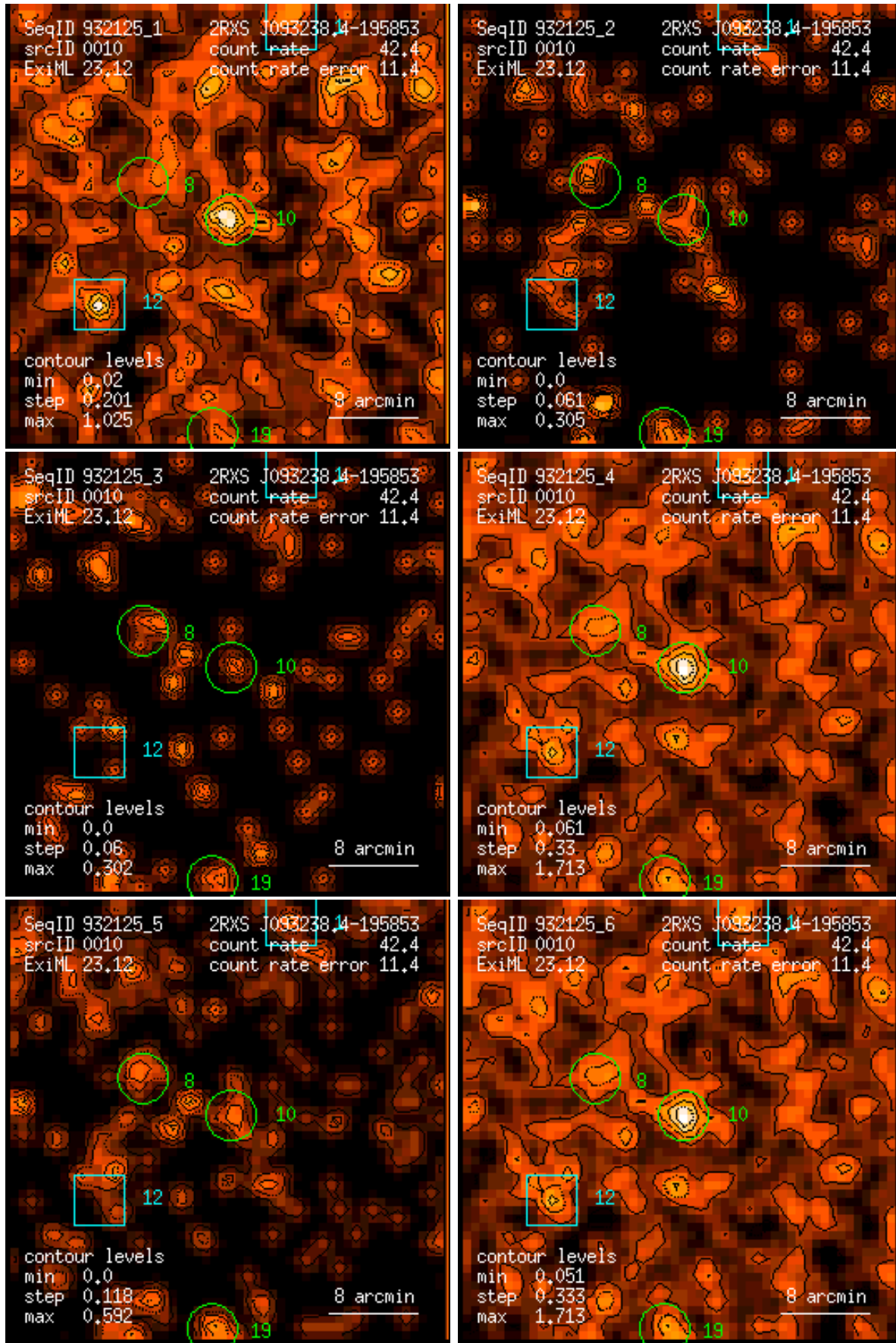
Figure 10: RASS 932125: detection 0010: band rate images, Gaussian filter: (1) PSPC channels 11 – 41, (2) 52 – 90, (3) 91 – 201, (4) 11 – 235, (5) 52 – 201, (6) 11 – 201. Broad band rates in counts/ks. Band rate contour levels in counts/ks/arcmin 2 .
