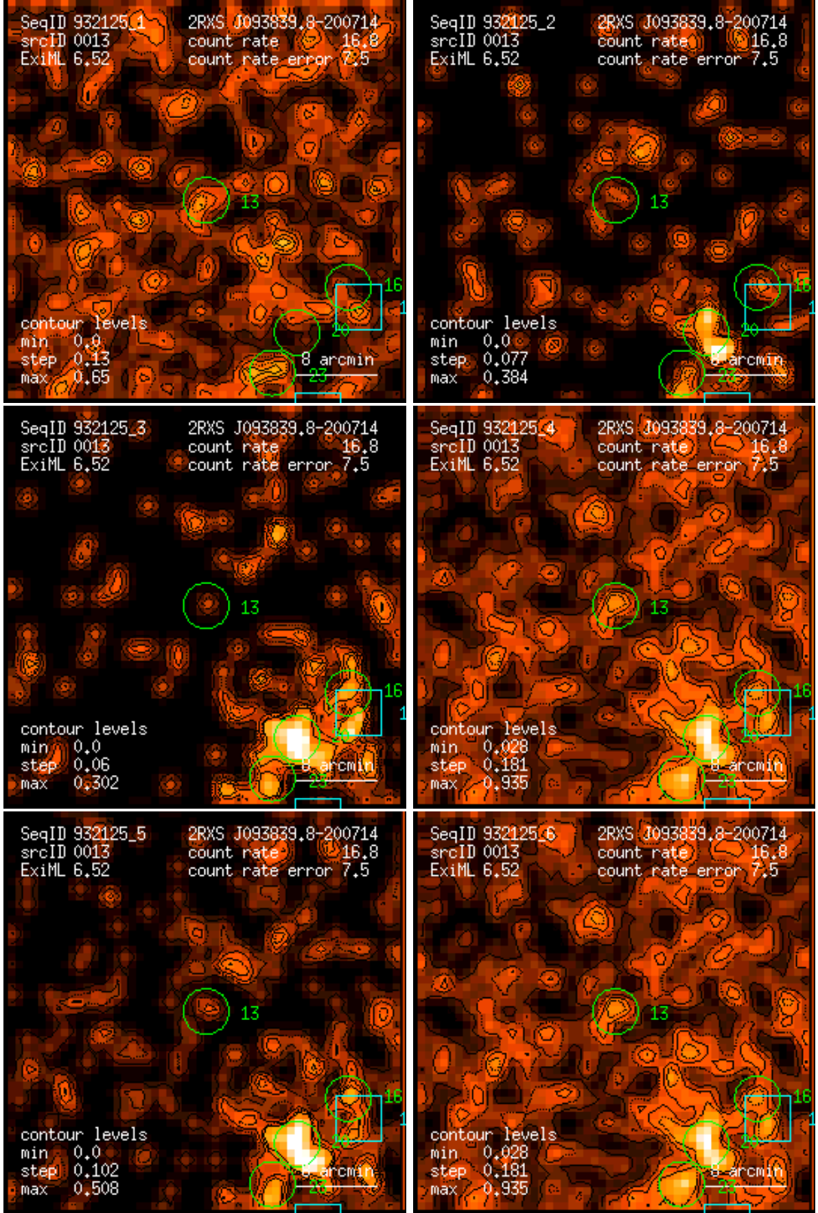
Figure 13: RASS 932125: detection 0013: band rate images, Gaussian filter: (1) PSPC channels 11 – 41, (2) 52 – 90, (3) 91 – 201, (4) 11 – 235, (5) 52 – 201, (6) 11 – 201. Broad band rates in counts/ks. Band rate contour levels in counts/ks/arcmin 2 .
