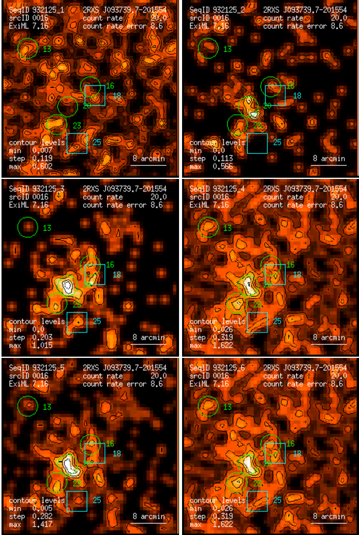
Figure 16: RASS 932125: detection 0016: band rate images, Gaussian filter: (1) PSPC channels 11 – 41, (2) 52 – 90, (3) 91 – 201, (4) 11 – 235, (5) 52 – 201, (6) 11 – 201. Broad band rates in counts/ks. Band rate contour levels in counts/ks/arcmin 2 .
