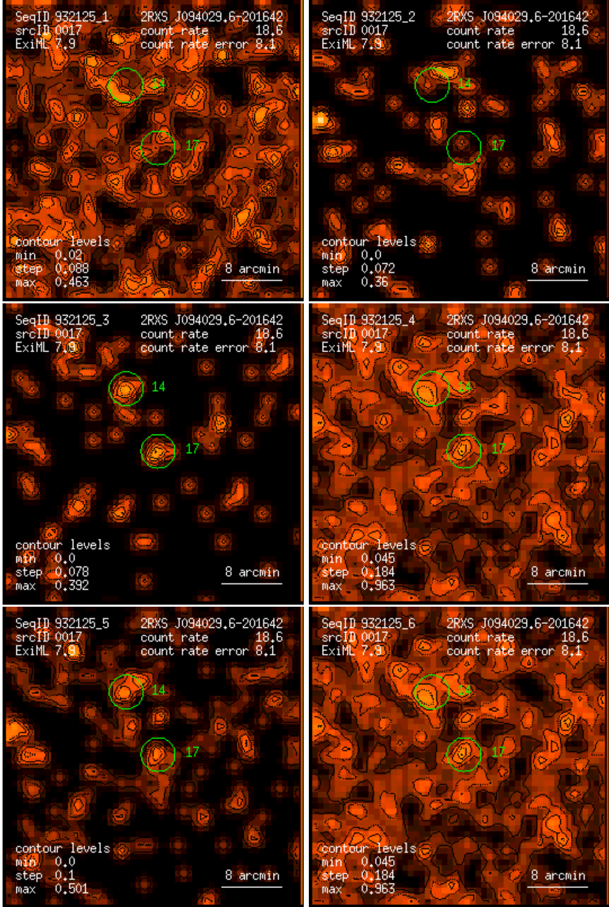
Figure 17: RASS 932125: detection 0017: band rate images, Gaussian filter: (1) PSPC channels 11 – 41, (2) 52 – 90, (3) 91 – 201, (4) 11 – 235, (5) 52 – 201, (6) 11 – 201. Broad band rates in counts/ks. Band rate contour levels in counts/ks/arcmin 2 .
