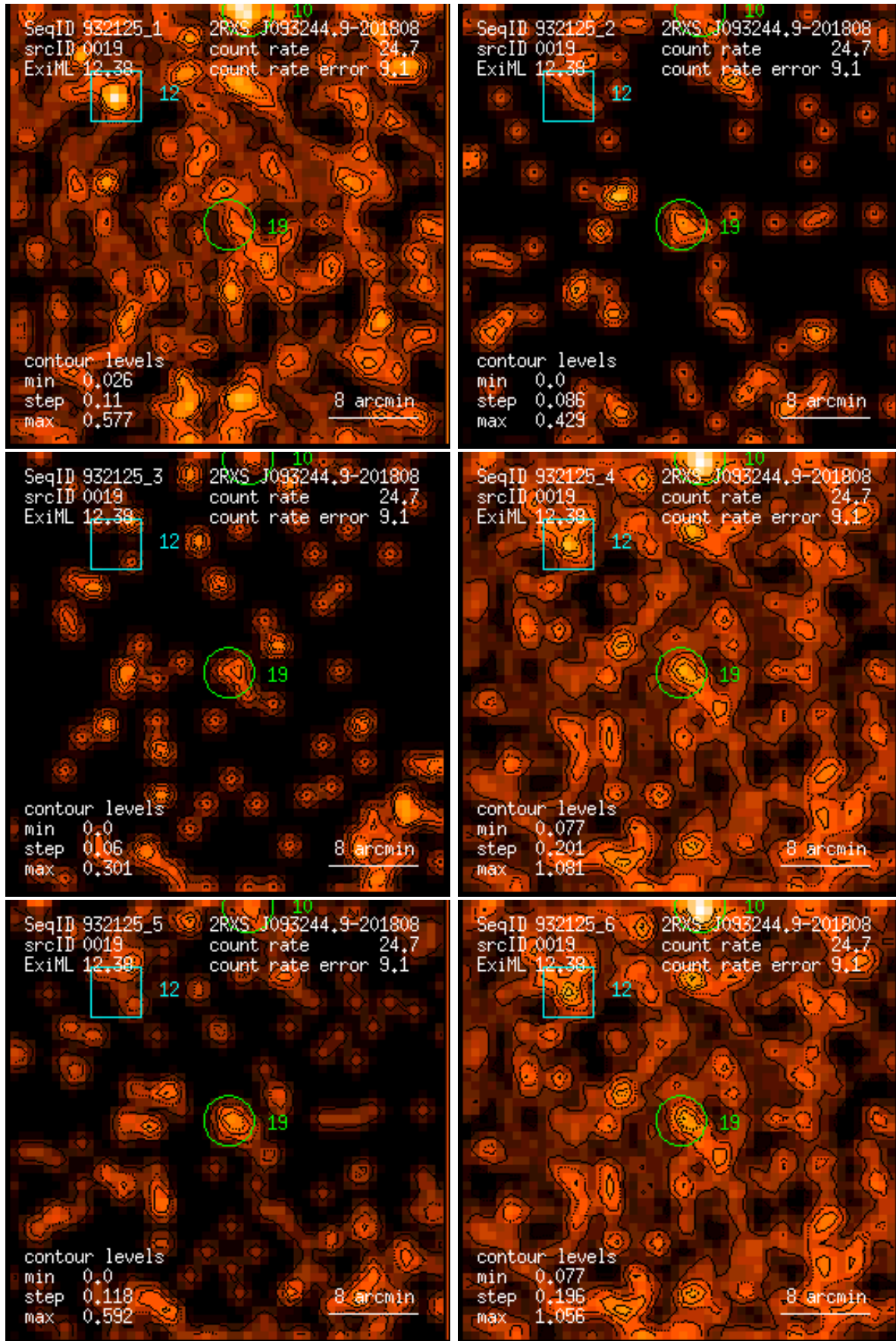
Figure 19: RASS 932125: detection 0019: band rate images, Gaussian filter: (1) PSPC channels 11 – 41, (2) 52 – 90, (3) 91 – 201, (4) 11 – 235, (5) 52 – 201, (6) 11 – 201. Broad band rates in counts/ks. Band rate contour levels in counts/ks/arcmin 2 .
