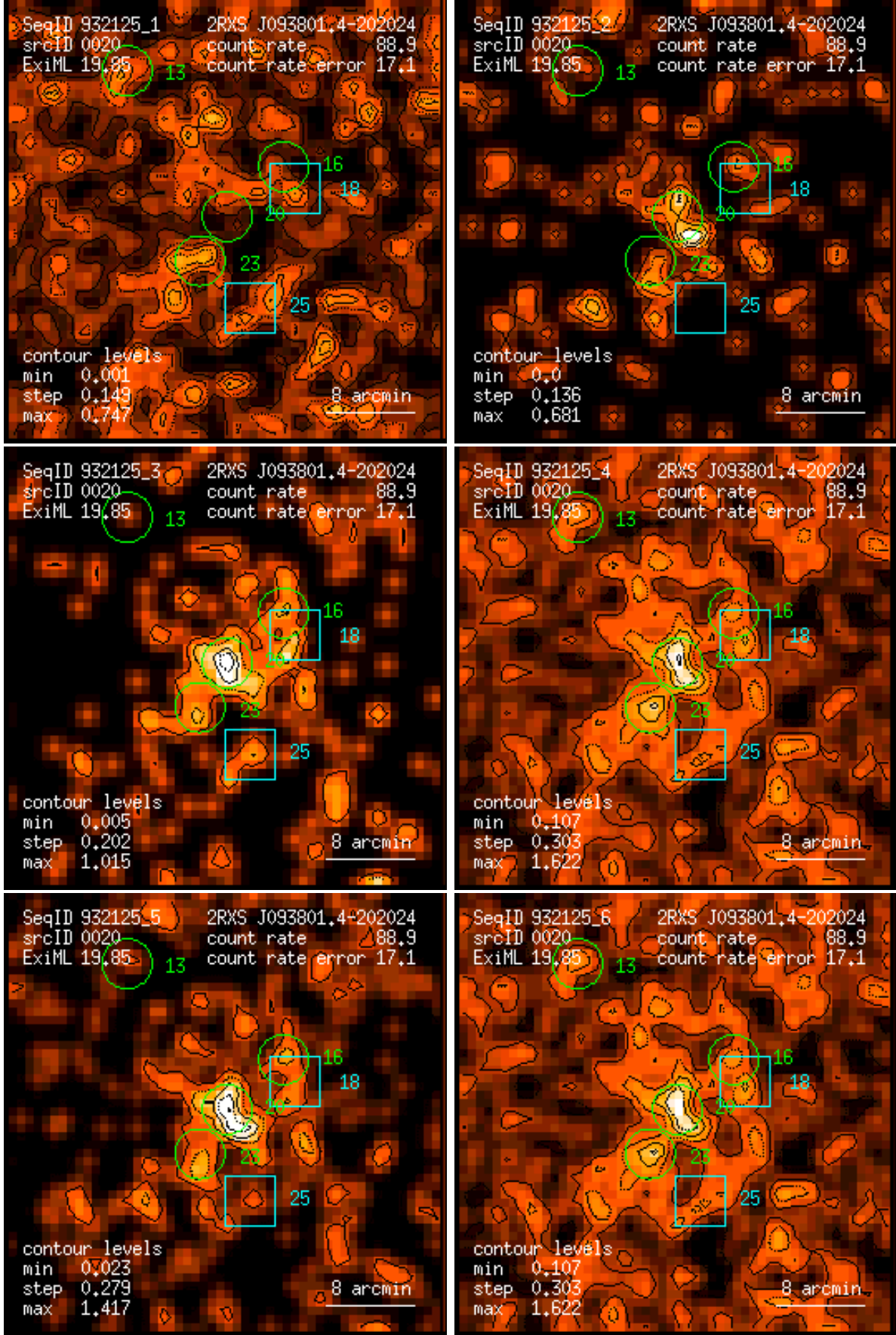
Figure 20: RASS 932125: detection 0020: band rate images, Gaussian filter: (1) PSPC channels 11 – 41, (2) 52 – 90, (3) 91 – 201, (4) 11 – 235, (5) 52 – 201, (6) 11 – 201. Broad band rates in counts/ks. Band rate contour levels in counts/ks/arcmin 2 .
